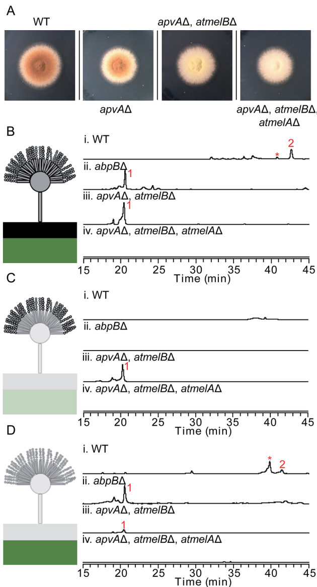
Fig. 3 (A) Phenotype of A. terreus wild type and other A. terreus mutant strains growing on LCM for 5 days. Morphological change of the fungal conidia can be observed if the deleted genes are involved in the biosynthesis of the brown conidial pigment. Total extracts (B), conidial extracts (C) and hyphal extracts (D) of A. terreus wild type and mutant strains as detected by UV at 370 nm. Aspulvinone related natural products are labeled in red. In B–D, the black box represents the top layer agar as described in tissue-specific extraction. The green box represents the bottom layer agar in tissue-specific extraction. The numbering of the peaks corresponds to the natural products shown in Fig. 2A. The aspulvinone E (1) and its related natural products can be detected in LC/MS traces Bi, Bii, Biii, Ciii, Di, Dii, and Diii. Trace amount of 1 identified in D iii is due to the diffusion of this compound synthesized in the conidia of the mutant strain. *This metabolite is related with aspulvinones according to its UV absorption and MS spectrum.
