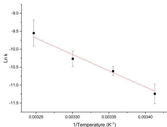
Fig. 4 Arrhenius plot for the determination of the activation energy for the esterification of one alcohol group of Ox063 by pyruvic acid, the slope as determined by the best fit was -9053.3 K. (see Fig. S2 and Table S1 for data points†).
