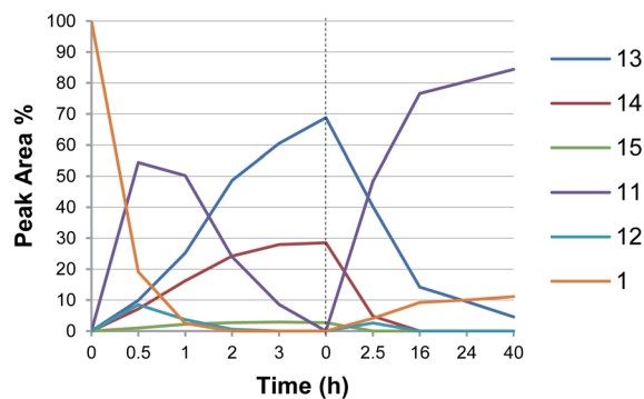
Scheme 3 De-Boc of di-Boc mixture to give 11 selectively. De-Boc conditions: n -BuNH 2 (1.5 equiv.), MTBE (8 mL g -1 ), 23 °C.
