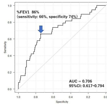
Figure 2 Receiver operating characteristic curve for progression from PRISm to COPD. The %FEV 1 cut-off for progression to COPD in subjects with a 1 s rate of 70% or greater (normal lung function group and PRISm). AUC, area under the curve; COPD, chronic obstructive pulmonary disease; FEV 1 , forced expiratory volume in 1 s; %FEV 1 , per cent forced expiratory volume in 1 s PRISm, preserved ratio impaired spirometry.
