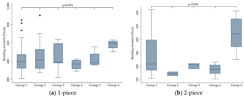
Figure 10. Boxplots showing the bending moment at the time point of fracture depending on dynamic loading conditions respecting the applied load and amount of cycles (as categorized in Section 2.7) for 1- (a) and 2-piece (b) zirconia implants. Whiskers are used to represent all samples lying within 1.5 times the interquartile range. Dots represent outliers. Detailed data can be found in Tables 3 and 4. No 2-piece implants were allocated to group 5.
