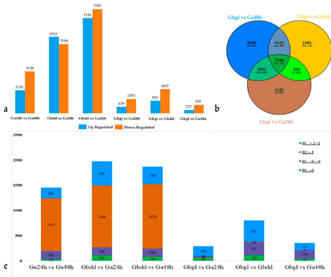
Figure 3. Expression dynamics changes and comparative analysis of differentially-expressed genes (DEGs) between Gbgl, Ga24h, Gbdd and Ga48h following delayed gland morphogenesis at imbibed seed and seedling stages. (a) Number of DEGs showing the up-regulated and down-regulated genes; (b) Venn diagram showing common genes, all differentially-expressed genes in different stages; (c) the number of transcripts demonstrating changes in expression in Gbgl, Ga24h, Gbdd and Ga24h following pattern fold change (FC) in expression, calculated as the log 2 ratio of gene expression in glandless imbibed seed with glanded imbibed seed and seedling. Gbdd, Ga24h, Gbgl and Ga48h represent G. bickii glanded seedlings, G. arboreum glanded imbibed seeds, G. bickii glandless imbibed seeds and G. arboreum glanded seedlings, respectively.
