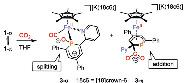
Scheme 2. Reaction of 1- \sigma and 1- \pi with CO 2 (1 atm) in THF at room temperature.
