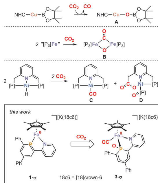
Figure 1. C=O cleavage in CO 2 mediated by well-defined late 3d metal complexes. NHC = N-heterocyclic carbene. [P_3] = PhB(CH_2P(CH_2CH_2)_2)_3 . [P] = P^iPr_2 .
