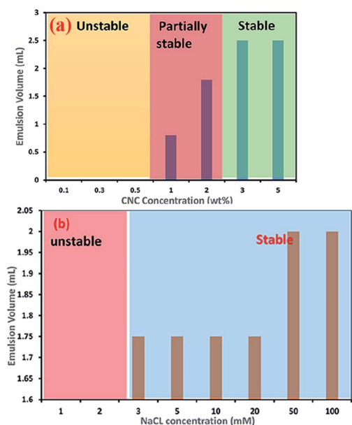
Fig. 4 Effect of (a) CNC concentration and (b) addition of NaCl to a 0.1 wt% CNC suspension on the stability of O/W Pickering emulsions. 32 Reprinted from ref. 32, Copyright 2018, under the terms of the CC BY License, published in the Frontiers in Chemistry .
