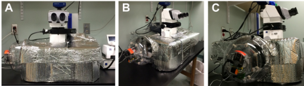
Figure 4. Self-constructed heated incubation chamber. (A-C) Shown is a heated incubation chamber made of cardboard, bubble wrap and Velcro. A wired dome heater (originally designed for chicken egg incubation) is attached to the chamber using aluminum tape. Please click here to view a larger version of this figure.
