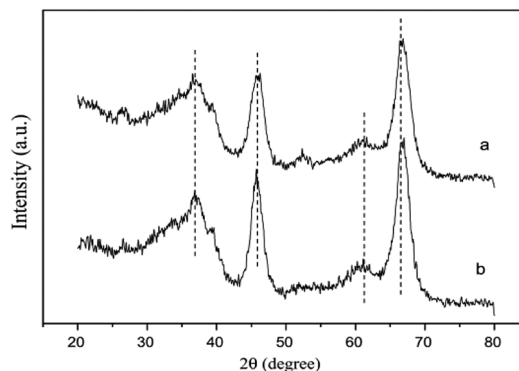
Fig. 10 XRD patterns of two different \text{SnO}_2 - \text{Al}_2\text{O}_3 catalysts: (a) \text{Sn}^5 (IM) and (b) \text{Sn}^5 (SG). 42
