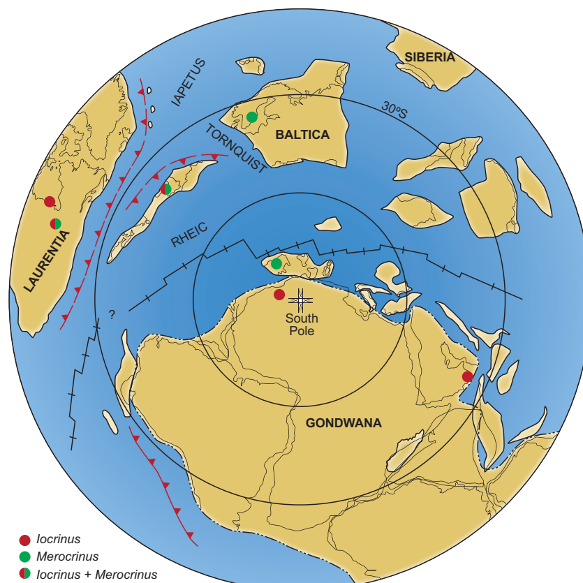
Figure 6 Distribution of the major paleocontinents during the Middle Ordovician, showing the known geographical distribution of Iocrinus and Merocrinus . Locality markers indicate the presence of a taxon on a palaeocontinent; multiple localities are not noted on a single palaeocontinent. Modified from Cocks & Torsvik (2006) .
