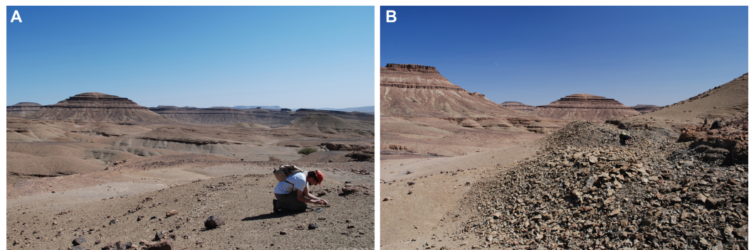
Figure 3 Field photographs showing the Taddrist Formation and the levels yielding fossiliferous concretions. (A) General view of the Taddrist Formation in the studied area. (B) Detail of the trench providing the fossiliferous concretions.
