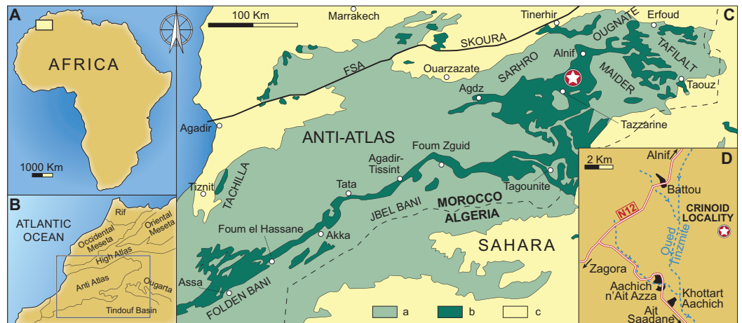
Figure 2 Geographical and geological setting of the eastern Anti-Atlas Mountains, Morocco, showing the type locality of the new species (indicated by a star) close to the village of Battou. After Rábano, Gutiérrez-Marco & García-Bellido (2014) . (A) Map of Africa. (B) Detailed map of west Africa showing the position of the Anti-Atlas Mountains. (C) Simplified geological map of Morocco with the position of the studied locality; a: Precambrian and Palaeozoic rocks, b: Ordovician rocks, c: post-Palaeozoic cover. (D) Geographic map indicating the position of the studied locality.
