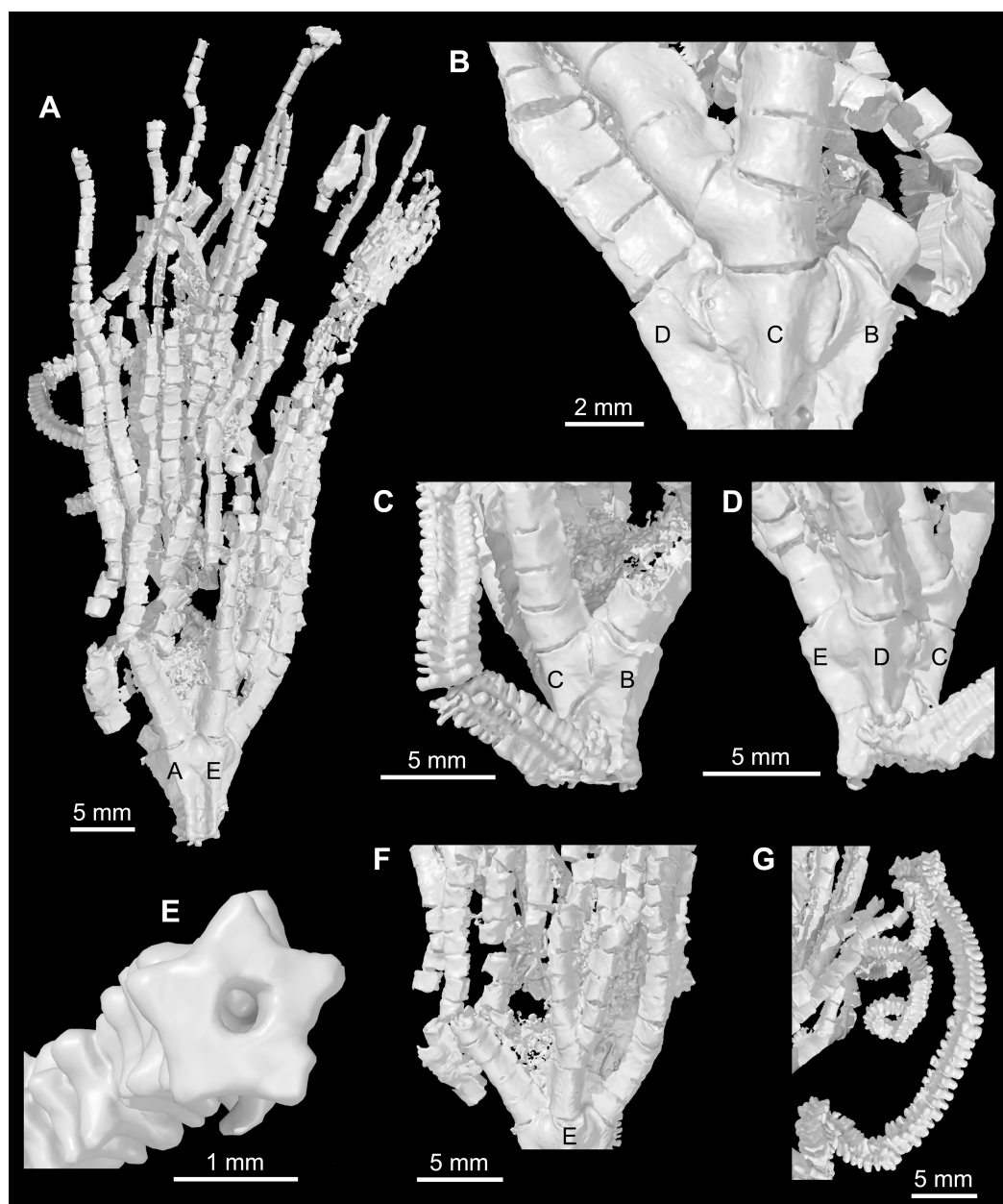
Figure 5 Iocrinus africanus sp. nov. (MGM 6754) from the Darriwilian (Middle Ordovician) of Morocco. Digital reconstructions of the specimen. (A) General morphology showing the AE-interray. (B) Detail of the theca showing the C-ray. (C) Detail of the cup showing the BC-interray. (D) Detail of the cup showing the D-ray. (E) Detail of the column showing pentastellate shape and holomeric construction. (F) Detail of the proximal arms showing the E-ray. (G) Column in an open coil. Abbreviations: A–E, ambulacra.
