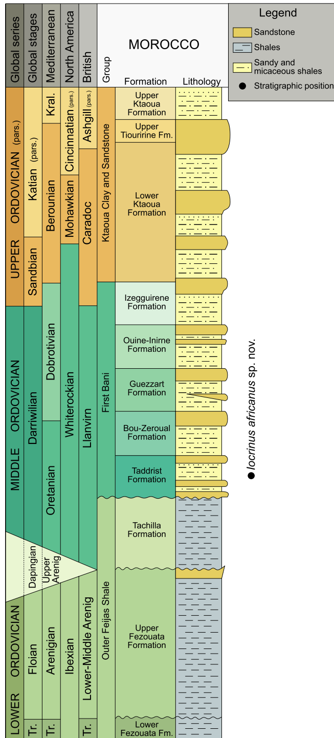
Figure 1 Chronostratigraphical chart for the Ordovician, indicating the levels that provided the studied specimen. Correlations between stratigraphical units in the Anti-Atlas (after Destombes, Hollard & Willefert, 1985; Gutiérrez-Marco et al., 2003; Villas et al., 2006 ), the British regional time scale ( Fortey et al., 1995 ), North American graptolite zonal sequences ( Webby et al., 2004 ), Mediterranean regional stages ( Gutiérrez-Marco et al., 2003 ), and global stages are shown. Modified from Sumrall & Zamora (2011) . Abbreviations: Kral, Kralodvorian; pars., partial; Tr., Tremadocian.
