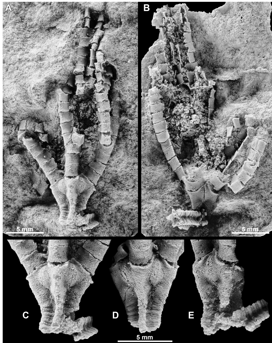
Figure 4 Iocrinus africanus sp. nov. (MGM 6754) from the Darriwilian (Middle Ordovician) of Morocco. (A), (B) General morphology including the complete crown showing the E-ray (A) and BC-interray (B), the proximal column, and part of the arms. (C) Detail of the cup showing the E-ray. (D) Detail of the cup showing the A-ray. (E) Detail of the cup showing the D-ray. All images are photographs of latex casts of the specimen whitened with ammonium chloride sublimate.
