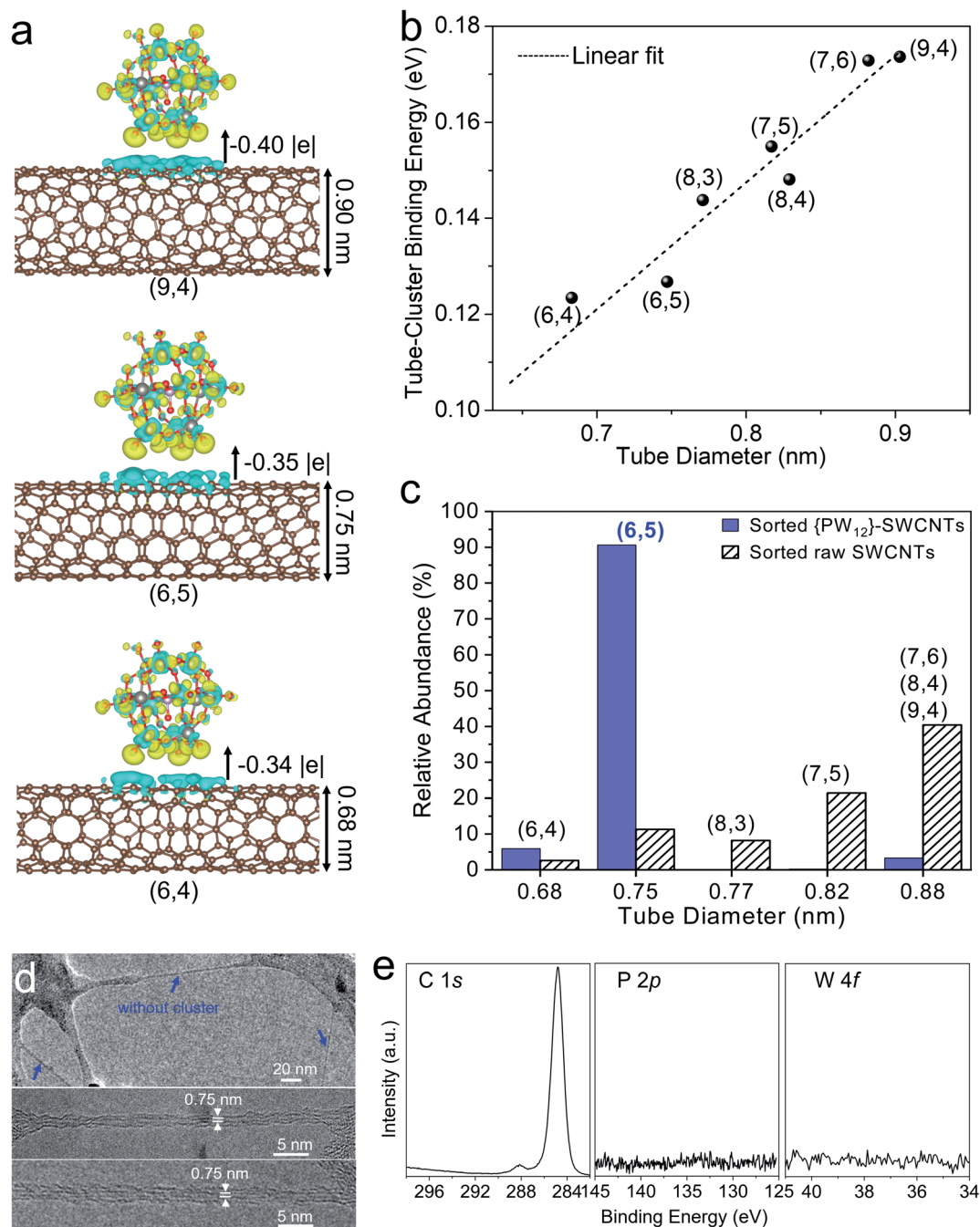
Fig. 3 (a) DFT calculations: iso-surface plots of the electron density differences for \{PW_{12}\} on the outside of SWCNTs with different chiralities/diameters: (6,4), (6,5), and (9,4). The corresponding electron transfer ( |e| ) is indicated. (b) Binding energy of (n,m) SWCNTs with \{PW_{12}\} . The fitting line gives y = 0.26x - 0.06 , with an R^2 = 0.96 , and shows a linear correlation between the tube diameter and binding energy. (c) Histogram showing the relative (n,m) abundance of PCz-sorted raw SWCNTs and \{PW_{12}\} -SWCNTs based on the absorption spectra. (d) TEM images of sorted \{PW_{12}\} -SWCNTs wrapped by the polymer. Blue arrows indicate the SWCNTs without clusters. (e) XPS spectra of the PCz-sorted \{PW_{12}\} -SWCNT film.
