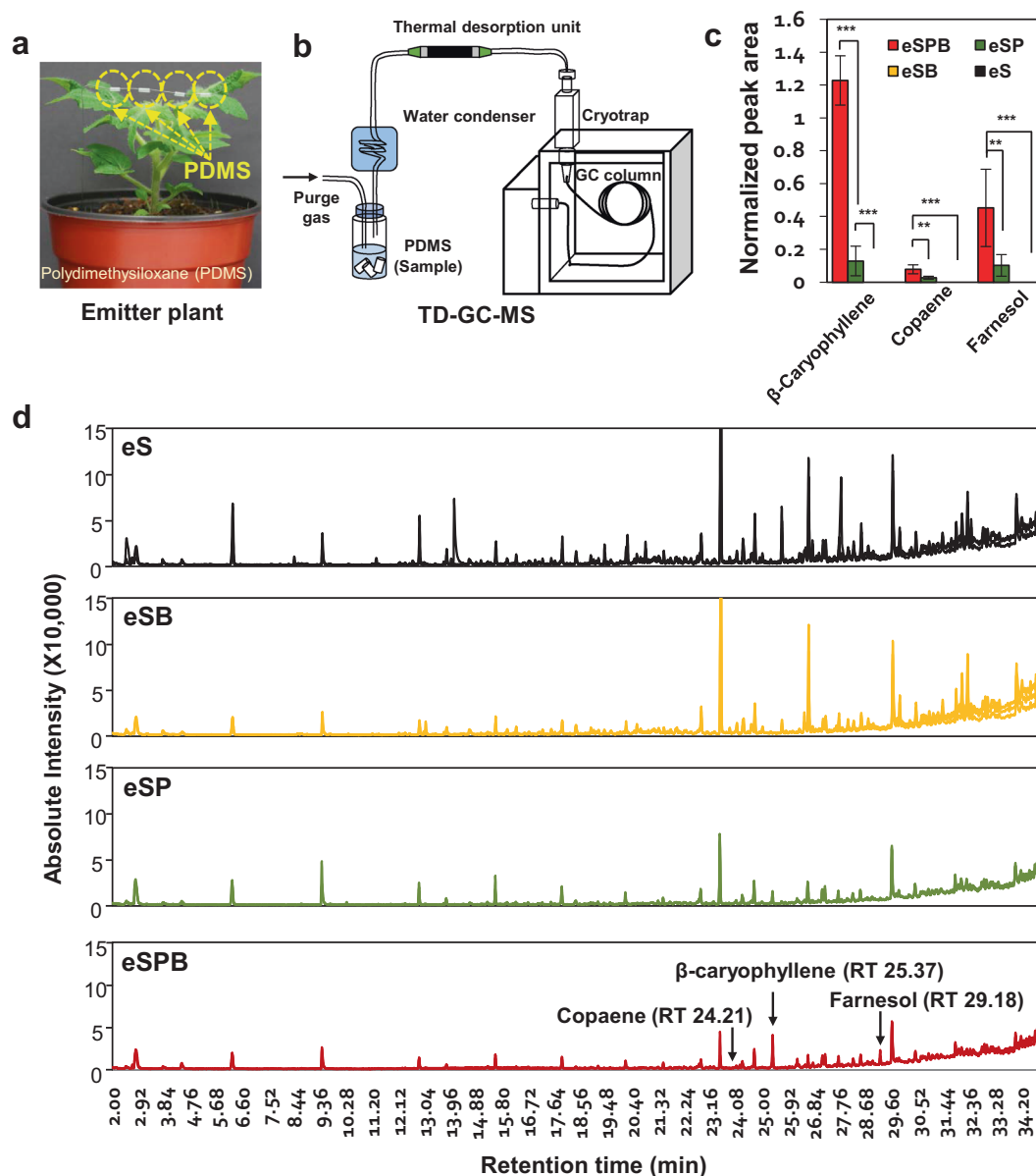
Fig. 4 Profiling of plant VOCs from an emitter plant treated with PGPR. a VOCs released aboveground by emitter plants collected via polydimethylsiloxane (PDMS) tubing pieces. b Schematic of a TD-GC-MS system for plant volatile analysis. c Three eSPB-specific volatiles selected on the basis of peak area (normalized relative to the PDMS derived peak). d Total ion chromatograms of VOCs released by
