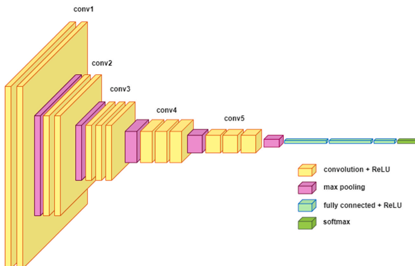
Fig. 10. VGG architecture.
