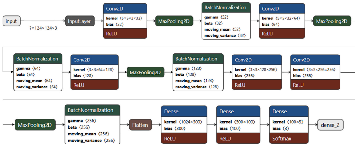
Fig. 7. AlexNet architecture.
