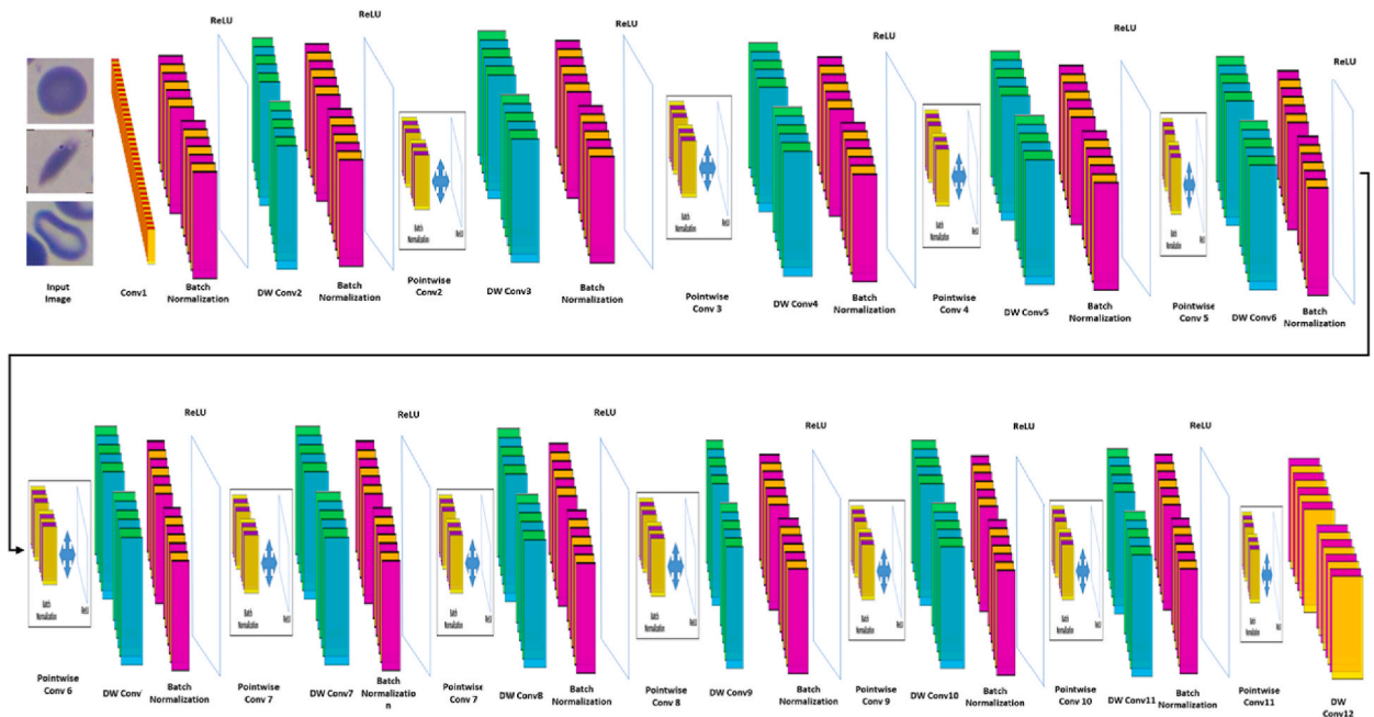
Fig. 12. MobileNet architecture.
