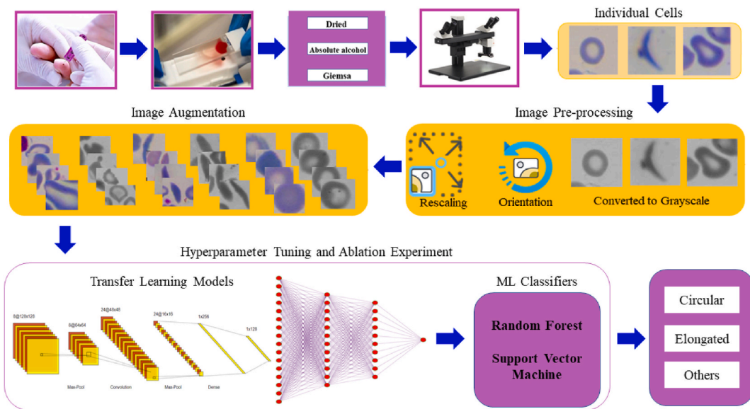
Fig. 4. A high-level overview of the proposed methodology.
