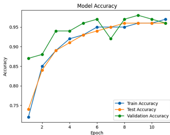
Fig. 9. Training, Testing, and Validation accuracy over time by AlexNet.
