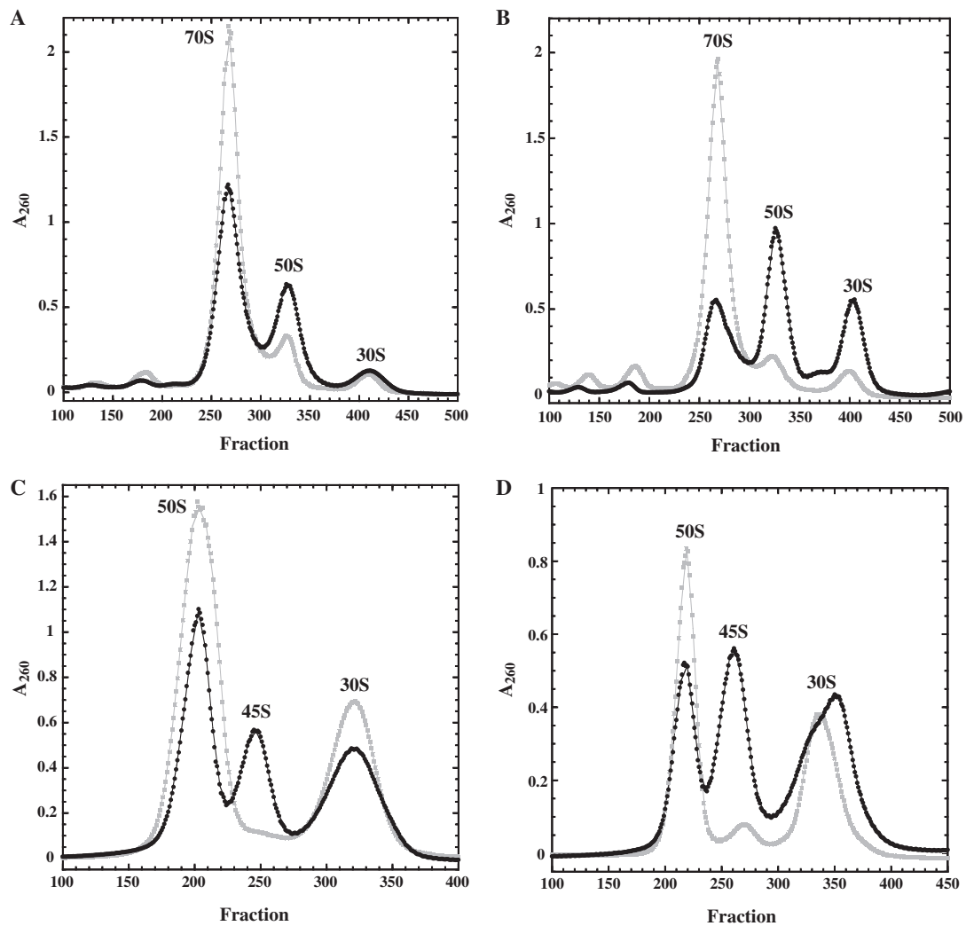
Figure 1. Ribosomes from cells overexpressing wild-type DbpA (grey squares) or the DbpA R331A mutant (black circles) grown at 37°C (A and C) or 22°C (B and D) and analyzed on gradients containing 10 mM Mg^{2+} , 10–50% sucrose (A and B) or 1 mM Mg^{2+} , 20–40% sucrose (C and D). Approximately, 1A 260 unit of ribosomes was loaded on each gradient.
