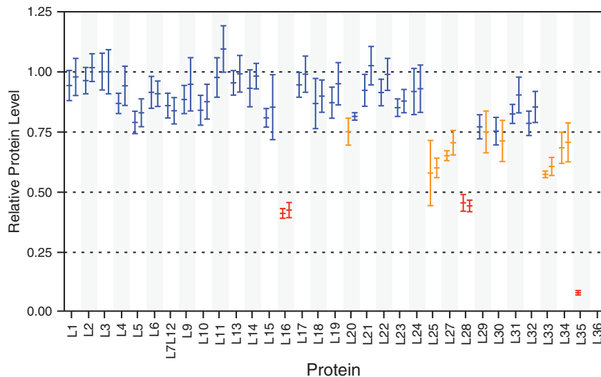
Figure 4. ESI-TOF MS analysis of the L-protein content of 45S particles from cells overexpressing DbpA R331A. Shown are the normalized relative protein levels compared to wild-type 50S subunits for two sample replicates. Proteins present at near-native levels are shown in blue, proteins present at moderately decreased levels are shown in orange, and proteins present at significantly decreased levels are shown in red. Error bars indicate differences in measurements obtained for multiple peptides from the same protein. No data was obtained for L36.
