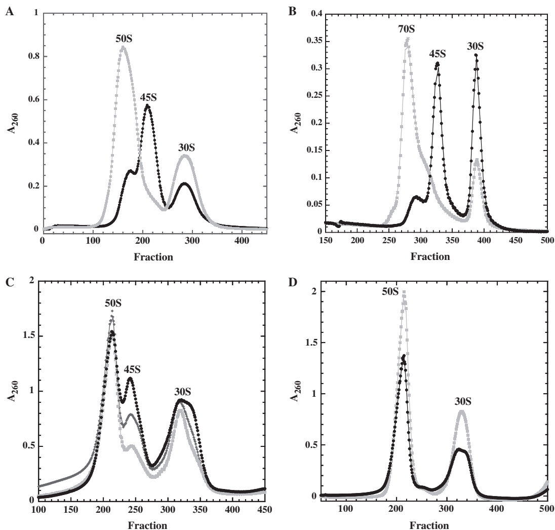
Figure 2. (A) DbpA R331A 50S subunits (black circles) and 70S ribosomes (grey squares) collected from gradients containing 10 mM Mg^{2+} analyzed on a second gradient containing 1 mM Mg^{2+} . (B) DbpA R331A 50S (grey circles) and R331A 45S (black circles) incubated with native 30S subunits and analyzed on gradients containing 10 mM Mg^{2+} . (C) Ribosomes from cells overexpressing DbpA mutants, DbpA R331A (black circles), DbpAK53A (dark grey diamonds) or DbpA E154A (grey squares) were analyzed on sucrose gradients containing 1 mM Mg^{2+} . (D) BL21(DE3) (grey squares) and BL21(DE3) \Delta dbpA (black circles) were grown to midlog at 22°C and analyzed on sucrose gradients containing 1 mM Mg^{2+} .
