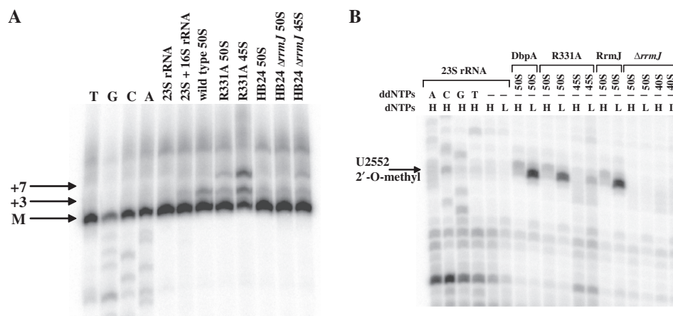
Figure 3. RNA from wild-type DbpA 50S subunits, DbpA R331A 50S subunits, DbpA R331A 45S particles, RrmJ 50S subunits, \Delta rrmJ 50S subunits and \Delta rrmJ 40S particles was analyzed by primer extension using 5'-end labeled primers 1 and 2. (A) The positions of the mature 5'-end (M) of 23S rRNA and the longer products (+3 and +7) of pre-23S rRNA are as indicated. (B) Primer 2 is complementary to nucleotides 3' of hairpin 92 of 23S rRNA and permits detection of the 2'-O-methyl at U2552 by reverse transcription in the presence of low dNTP concentration. H and L indicate high (1 mM) and low (4 \mu M) dNTP concentrations. Primer extension stops at modification sites are seen as bands in the low dNTP lanes. On both gels, the first four lanes show a sequencing ladder obtained using the same primers and 23S rRNA transcript. Control experiments were performed with 23S rRNA transcript and 23S + 16S rRNA purified from MRE600 cells.
