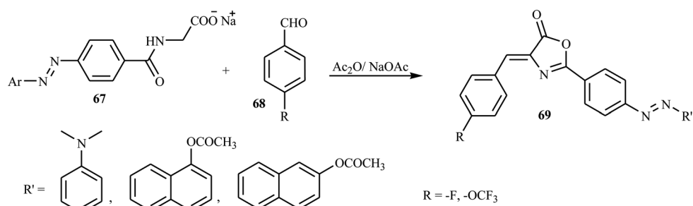
Scheme 16 General synthesis route towards azo dye derivatives containing oxazolone 69.
