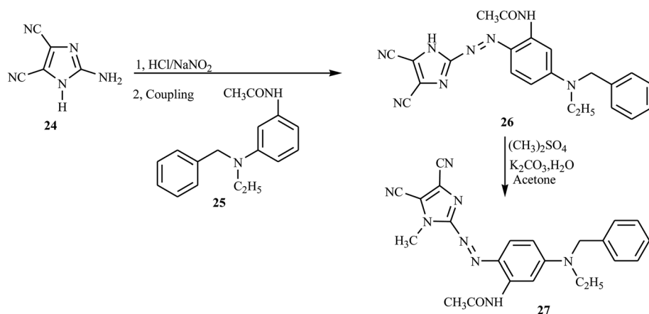
Scheme 5 General synthesis route towards azo dye derivatives containing imidazole 27 .
