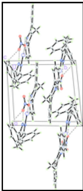
Fig. 2. The packing diagram of the title compound viewed down the c -axis. The dashed lines show the intermolecular interactions.
