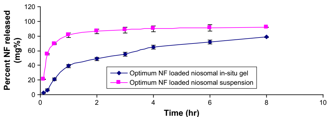
Figure S3 Release behavior of NF from NF-loaded niosomal suspension and NF-loaded niosomal in-situ gel (means \pm SD, n=3).
