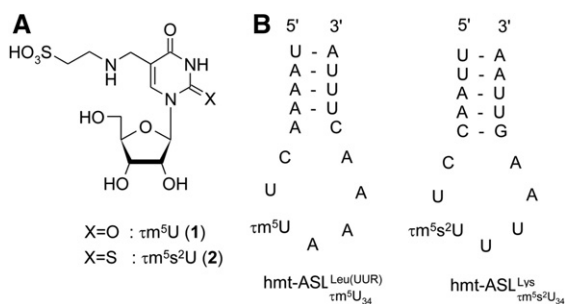
FIGURE 1. (A) The structure of 5-taurinomethyluridine ( \tau\text{m}^5\text{U} , 1 ) and 5-taurinomethyl-2-thiouridine ( \tau\text{m}^5\text{s}^2\text{U} , 2 ). (B) The sequence and secondary structure of the human mitochondrial tRNA Leu(UUR) and tRNA Lys anticodon stem and loop (hmt-ASL Leu(UUR) and hmt-ASL Lys ) bearing \tau\text{m}^5\text{U} and \tau\text{m}^5\text{s}^2\text{U} , respectively. The native sequence of hmt-ASL Leu(UUR) has pseudouridine ( \Psi ) at position 27, while in the sequence of hmt-ASL Lys there are two pseudouridines ( \Psi ) at positions 27 and 28, and N -[(9- \beta -D-ribofuranosyl-9 H -purin-6-yl)carbamoyl]-L-threonine ( \text{t}^6\text{A} ) at position 37.
