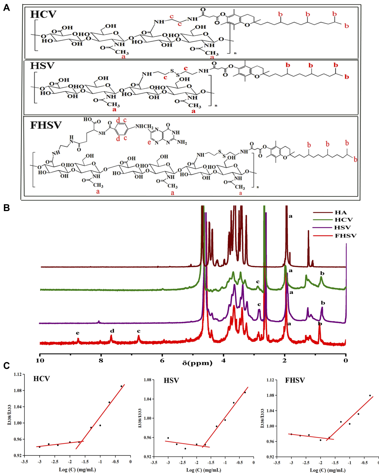
Figure 2 (A) Chemical structures of HCV, HSV and FHSV polymers. (B) 1 H-NMR spectra of HA in D 2 O, HCV, HSV and FHSV polymers in DMSO- d 6 /D 2 O (v/v, 1:1). (C) The CMC of HCV, HSV and FHSV polymers.
