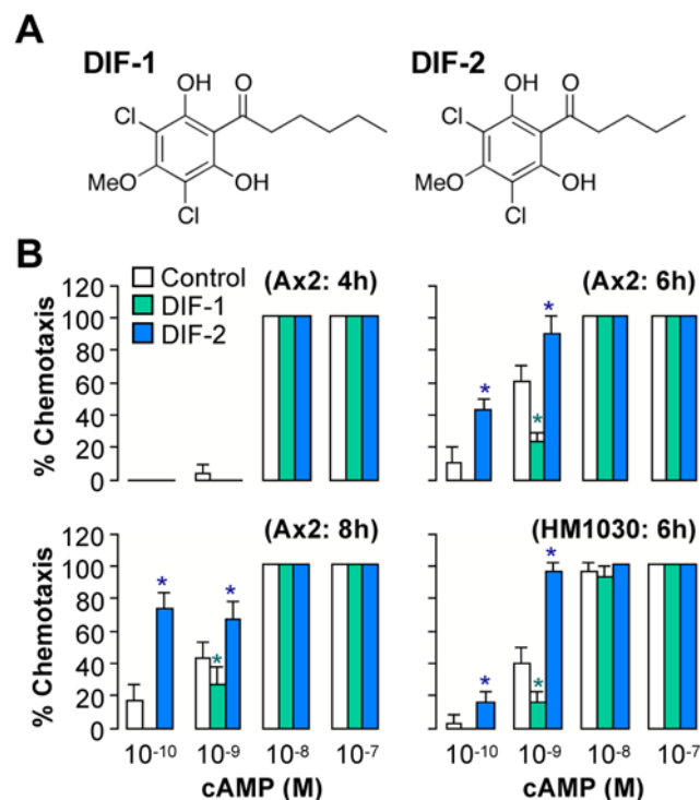
Figure 1. Effects of DIF-1 and DIF-2 on chemotaxis in Ax2 and HM1030 ( dmtA ) cells. (A) Chemical structure of DIF-1: 1-(3,5-dichloro-2,6-dihydroxy-4-methoxyphenyl)hexan-1-one and DIF-2: 1-(3,5-dichloro-2,6-dihydroxy-4-methoxyphenyl)pentan-1-one. (B) Ax2 and HM1030 cells were starved for 4–8 h (as indicated in parentheses) in shake-culture, and cell droplets were spotted on PB agar containing 3 mM caffeine (Control) plus 100 nM DIF-1 or DIF-2. Cells were assayed for chemotaxis toward the indicated doses of cAMP (10 cell droplets were examined for each cAMP concentration). Data are the mean and s.d. (bars) of three independent experiments (n = 3). * P < 0.05 , as compared with Control.
