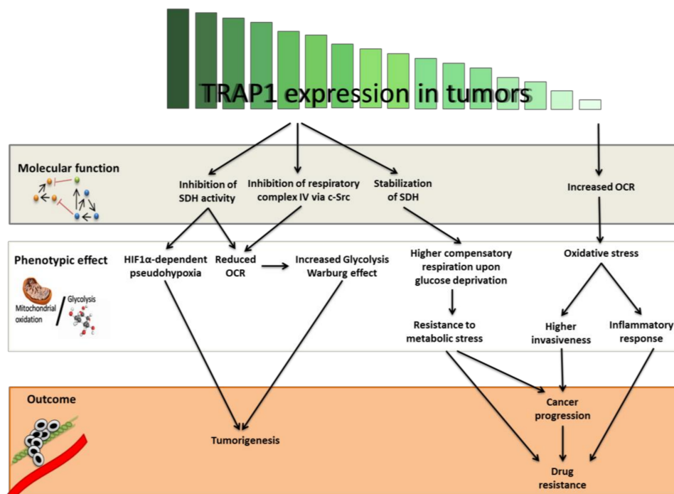
Figure 1. Hierarchical effects of Tumor Necrosis Factor Receptor-associated Protein 1 (TRAP1) expression levels on tumor development and progression through the regulation of energetic metabolism. TRAP1 binds respiratory complexes in the mitochondrial matrix and regulates their activity, either directly or indirectly via c-Src (grey box). This regulation alternatively leads to (i) a switch toward a more glycolytic (Warburg) phenotype, (ii) an enhanced ability to handle metabolic stress through the use of spare respiratory capacity and (iii) increased oxidative stress (white box). As a result, tumors with high glycolytic metabolism or limiting nutrient availability may gain the advantage of a high TRAP1 expression. Conversely, tumors mostly relying on oxidative metabolism may counter-select TRAP1 expression for progression and development of resistance and metastases (orange box). OCR: oxygen consumption rate; SDH: Succinate dehydrogenase; c-Src: SRC Proto-Oncogene; HIF1 \alpha : Hypoxia Inducible Factor 1 Alpha Subunit.
