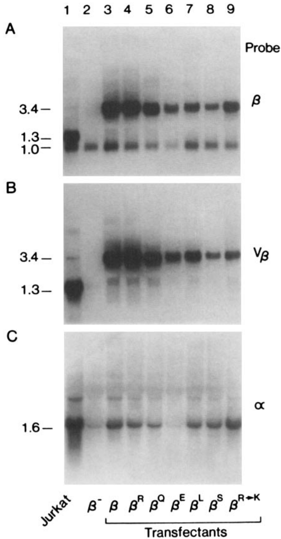
FIGURE 2. Northern blots of RNA isolated from Jurkat cells (lane 1), \beta chain-deficient mutant J.RT3-T3.5, which served as the recipient in transfections (lane 2), and transfectants (lanes 3-9). A single letter superscript is used to designate the mutations at position 290 from the wild-type lysine residue. The transfectant in lane 9 represents a cell transfected with cDNA in which the arginine 290 mutant cDNA served as a template to back-mutate that residue to lysine using the AAA codon. Blots were hybridized with a full-length Ti \beta chain cDNA probe (A), a V_{\beta} -specific cDNA probe (B) or a full-length Ti \alpha chain probe (C).
