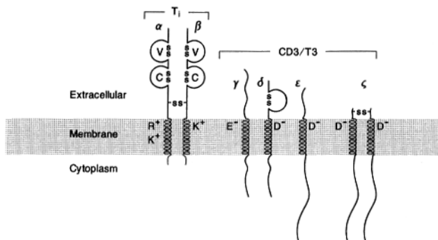
FIGURE 1. Schematic model of the human T cell antigen receptors. The single letter code for amino acids was used to designate charged residues within the membrane-spanning domains.
