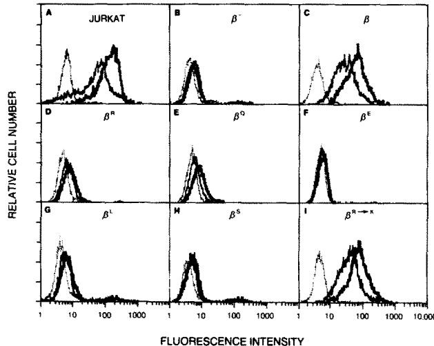
FIGURE 3. Flow cytometry histograms of Jurkat (A), \beta chain-deficient mutant J.RT3-T3.5 ( \beta^- ; B), which served as the recipient in transfections, and transfectants (C-I) stained with the following mAbs: IgG control (dotted lines); WT31, anti-Ti \alpha/\beta (thin solid lines); or anti-Leu-4, anti-CD3 (thick solid lines). A single letter superscript is used to denote the mutation at lysine 290 .
