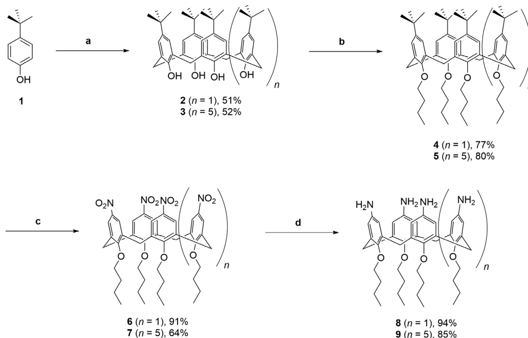
Scheme 1. Syntheses of calix[ n ]arenes 8 and 9. Reagents and reaction conditions: (a) n = 1 , (i) NaOH, 120 °C, 2 h, (ii) DPE, 120 °C, 1 h, (iii) 260 °C, 3 h (51%) or n = 5 , NaOH, 114 °C, 4 h, xylene (52%); (b) n = 1 , ^n\text{BuBr} , NaH, DMF, 60 °C, 24 h (77%) or n = 5 , ^n\text{BuBr} , NaH, KI, DMF, 40 °C, 72 h (80%); (c) n = 1 , \text{HNO}_3 , TFA, DCM, 1 h, rt (91%) or n = 5 , \text{NaNO}_3 , TFA, 7 h, rt (64%); (d) n = 1 , \text{H}_2\text{N-NH}_2\cdot\text{H}_2\text{O} , Pd/C (10%), EtOH, reflux, 48 h (94%) or n = 5 , \text{H}_2\text{N-NH}_2\cdot\text{H}_2\text{O} , Pd/C (10%), EtOH/THF, reflux, 24 h (86%).
