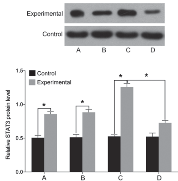
Figure 5. Detection of cell STAT3 levels by western blotting method. (A) Before miR-146a transfection. (B) miR-146a empty vector transfection. (C) miR-146a mimic transfection. (D) miR-146a inhibitor transfection. A comparison of STAT3 levels before and after treatment yielded no difference in the control group. The level of STAT3 is significantly higher in the experimental group than that in the control group before treatment. STAT3 level is increased after treatment with miR-146a mimic in the experimental group, and is decreased after treatment with miR-146a inhibitor. STAT3, signal transducer and activator of transcription 3; miR, microRNA. * P < 0.05 .
