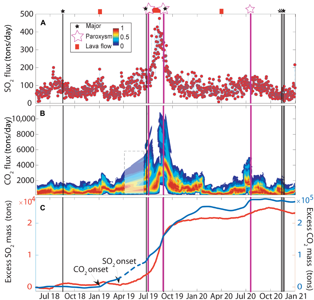
Fig. 4. Gas fluxes from the Stromboli's plume. Temporal record of daily averaged (A) \text{SO}_2 fluxes and (B) \text{CO}_2 fluxes. Data in (B) are calculated by multiplying the daily \text{CO}_2/\text{SO}_2 ratio frequency diagrams of Fig. 2C by the \text{SO}_2 fluxes of (A). Uncertainty in the derived \text{CO}_2 fluxes is evaluated at \leq 40\% from propagation of \text{CO}_2/\text{SO}_2 and \text{SO}_2 flux uncertainties. Gaps in the dataset (due to days of unsuccessful \text{CO}_2/\text{SO}_2 ratio determination because of the absence of plume fumigation at the Multi-GAS measurement site or Multi-GAS malfunctioning/failure) are filled by multiplying the measured \text{SO}_2 fluxes by \text{CO}_2/\text{SO}_2 ratios obtained from linear interpolation of the ratio time series (of Fig. 2C). These gaps are typically of a few days at most. Exceptions are the 9 April to 15 June 2019 [dashed area in (B)] and 4 to 21 July periods, in which the \text{CO}_2 flux results are based on data interpolation and should therefore be considered with caution. (C) Cumulative excess \text{SO}_2 (red) and \text{CO}_2 (blue) masses for the period from 10 May 2018 to 31 December 2020. The cumulative excess masses (see the main text) are obtained by subtracting the measured (A) and calculated (B) fluxes the pre-unrest phase (May to December 2018) time-averaged fluxes of 71 and 500 tons/day, respectively. Interpolated trends are identified by dashed lines. This plot suggests that accelerating \text{CO}_2 degassing regime is likely to have started in early 2019. Visible accelerations in the excess \text{CO}_2 are seen before both paroxysms.
