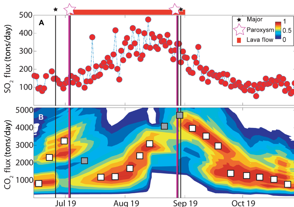
Fig. 5. A zoom of gas flux observations encompassing the summer 2019 effusive unrest. (A) \text{SO}_2 fluxes and (B) \text{CO}_2 fluxes. Squares in (B) identify weekly averaged median \text{CO}_2 fluxes (gray squares are for weeks in which no successful Multi-GAS measurements are available, and data interpolation was applied). The figure demonstrates two distinct \text{CO}_2 peaks before the two paroxysms. During the effusive event, a temporal lag is observed between \text{SO}_2 and \text{CO}_2 peaks. The 2019 effusive unrest thus involves (i) an initial period (3 July to 13 August) of rapid, efficient magma circulation in the upper conduits (high \text{SO}_2 ) and high lava output (67), followed by (ii) a second period (14 to 30 August) of vanishing shallow magma transport (declining \text{SO}_2 and magma effusion rates) [this study and (67)] but accelerating deep \text{CO}_2 degassing. Rapid drainage of conduit magma during 3 July to 13 August is thus a very likely causal factor for the 28 August paroxysm.
