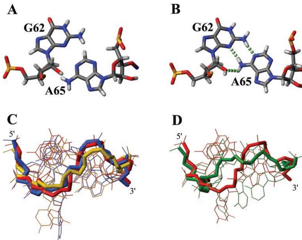
Figure 4. Structural features of the D-loop of BEVSLD. (A) The G62: synA65 ‘pseudo base pair’ as found in the experimentally determined mean structure of BEVSLDap. (B) The G62: synA65 base pair forming three hydrogen bonds (indicated as broken green lines) as derived from a 4 ns MD simulation using the calculated mean structure of BEVSLDap as starting structure. (C) Superimposition (backbone atoms of loop and closing base pair, top view) of the apical loop regions of the BEVSLDap structure (nt 61–66, red) with SLD of coxsackievirus B3 (uCACGg, blue, PDB 1RFR) and the TL1 tetraloop from 16S rRNA (cUUCGg, yellow, PDB 1F7Y). (D) Superimposition (backbone atoms of loop and closing base pair, top view) of the apical loop region of the BEVSLDap structure (nt 61–66, red) with the crystal structure of the cGUAAg tetraloop (blue, PDB 1MSY). The 5' and 3' ends of the tetraloop backbones are indicated.
