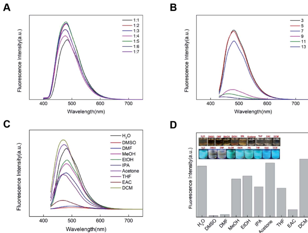
Fig. 4 (A) Fluorescence intensity of CDs solution and water diluted by different volume ratio; (B) fluorescence spectra of CDs with various pH; (C) fluorescence spectra of CDs with organic solvents; (D) fluorescence intensity histogram of CDs under the action of organic solvent and the pictures in daylight and ultraviolet light.
