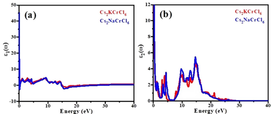
Fig. 5 Calculated plots of the (a) real part and (b) imaginary part of dielectric function versus the energy of Cs 2 KCrCl 6 and Cs 2 NaCrCl 6 perovskites.
