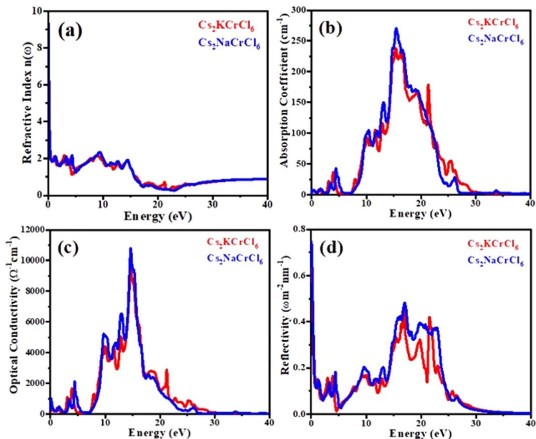
Fig. 6 Calculated plots of (a) refractive index, (b) absorption coefficient, (c) optical conductivity, and (d) reflectivity versus energy for Cs 2 KCrCl 6 and Cs 2 NaCrCl 6 perovskites.
