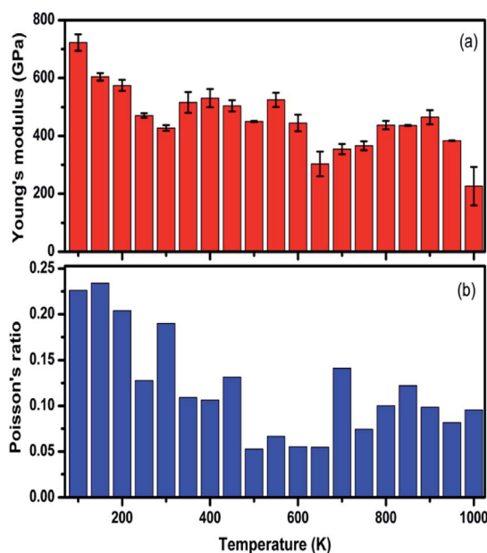
Fig. 5 The computed values for the (a) Young's modulus and (b) Poisson's ratio of graphene at various temperatures using the strain fluctuation method.
