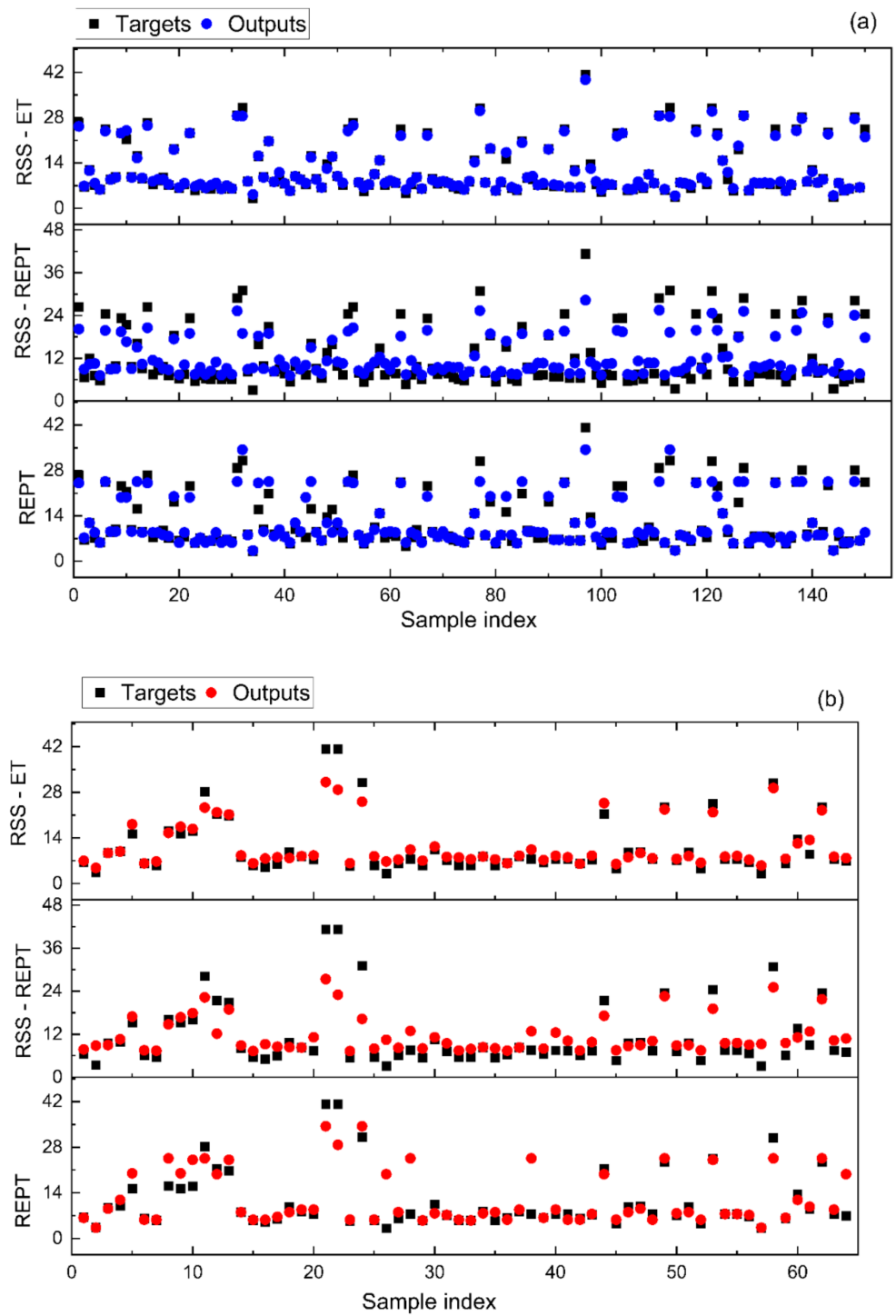
Figure 5. Comparison of the predicted and actual results: (a) Training and (b) test data.
