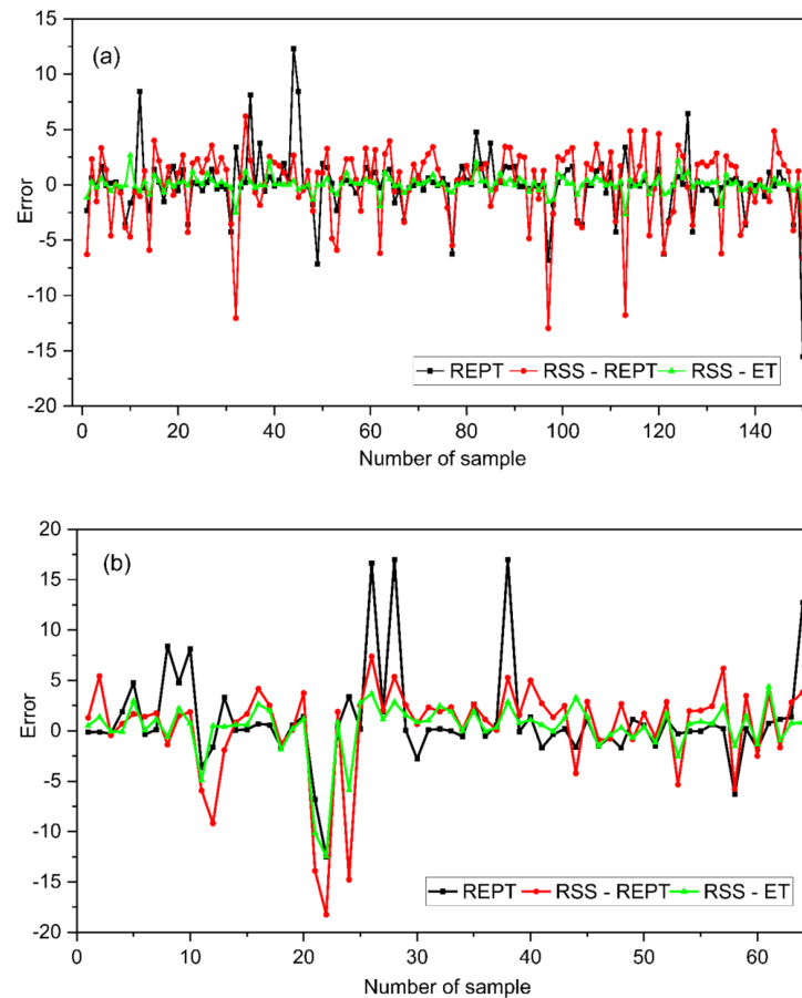
Figure 6. Error values for (a) training and (b) testing.
