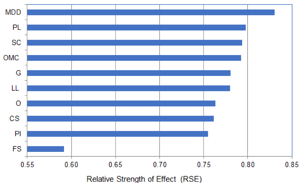
Figure 3. Sensitivity analysis of the input parameters predicting the CBR of soil.
