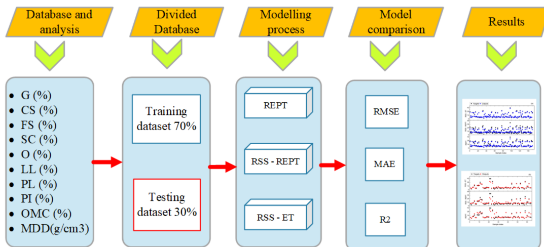
Figure 4. Methodological framework for the predicted values in this study.
