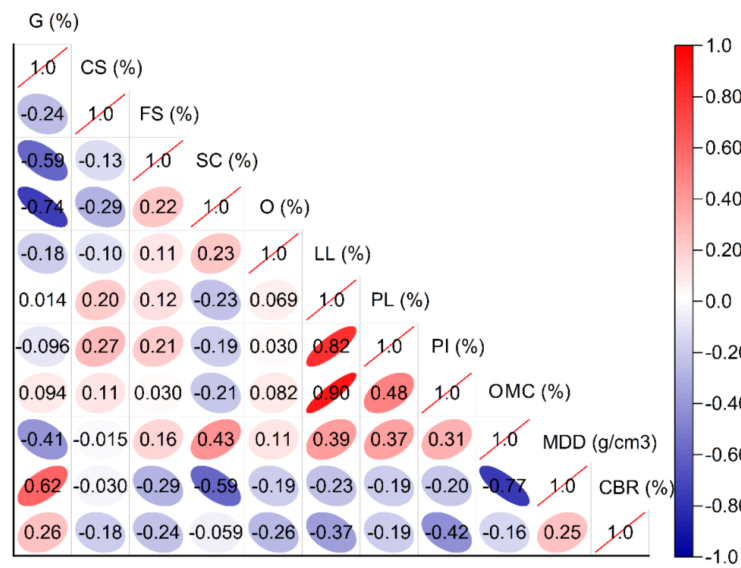
Figure 2. Correlation matrix analysis input variables in this study.
