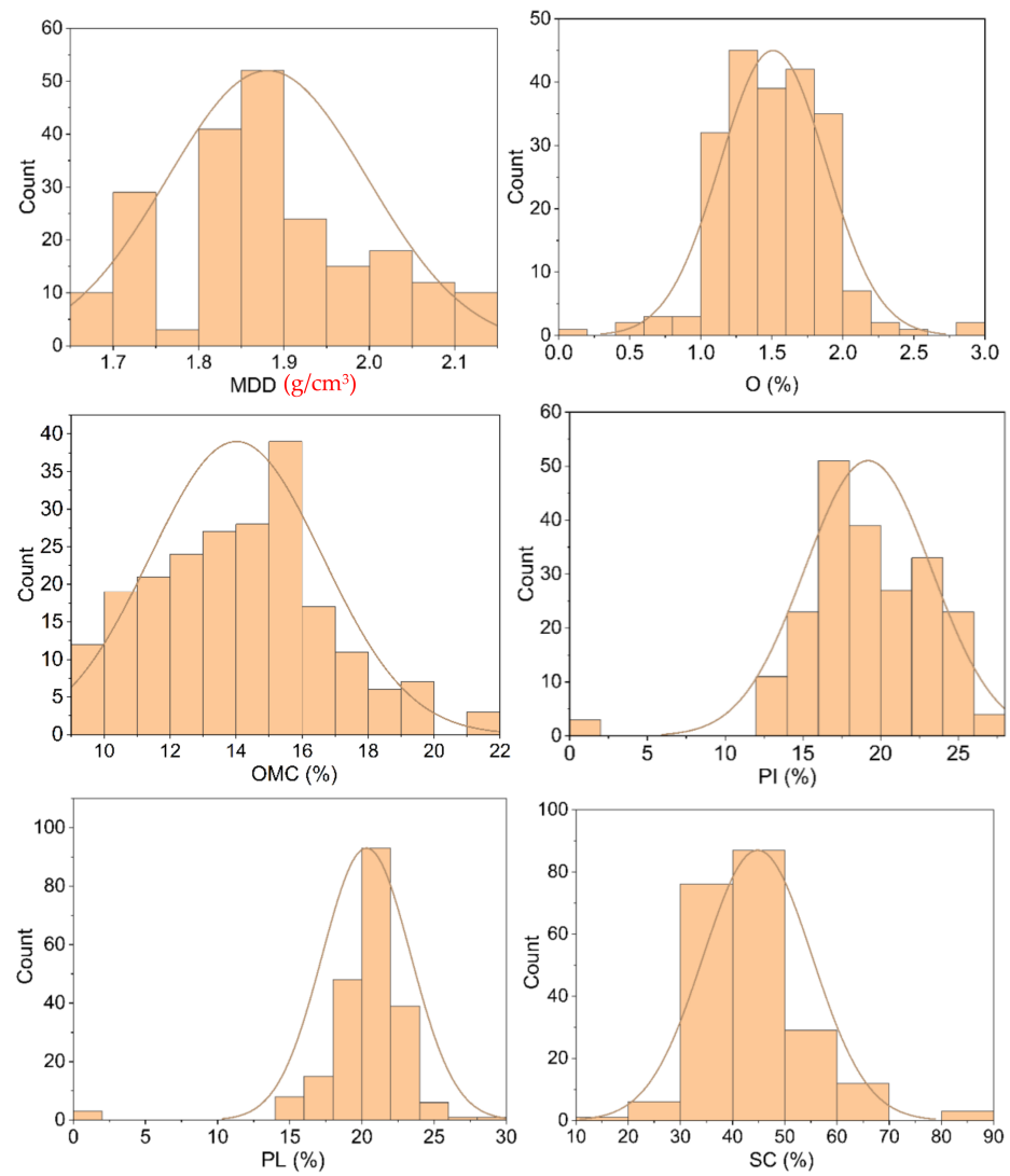
Figure 1. Statistical analysis distribution of the input parameters in this study.
