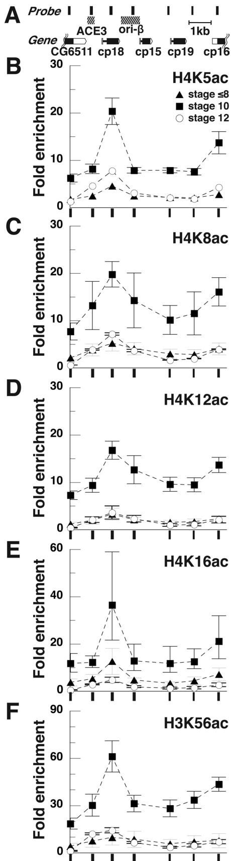
FIGURE 2: Developmentally dynamic acetylation of nucleosomes on multiple lysine residues correlates with activity of the DAFC-66D origin. (A) Diagram of DAFC-66D locus. Hatched boxes represent essential elements ACE3 and Ori- \beta (middle); the location of ChIP-
