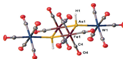
Figure 3. Molecular structure of 3 , with ellipsoids at 50% probability. Selected distances [Å]: As1–Fe1 2.4728(7), As1–Fe1' 2.4787(8), As1–W1 2.6380(5).
