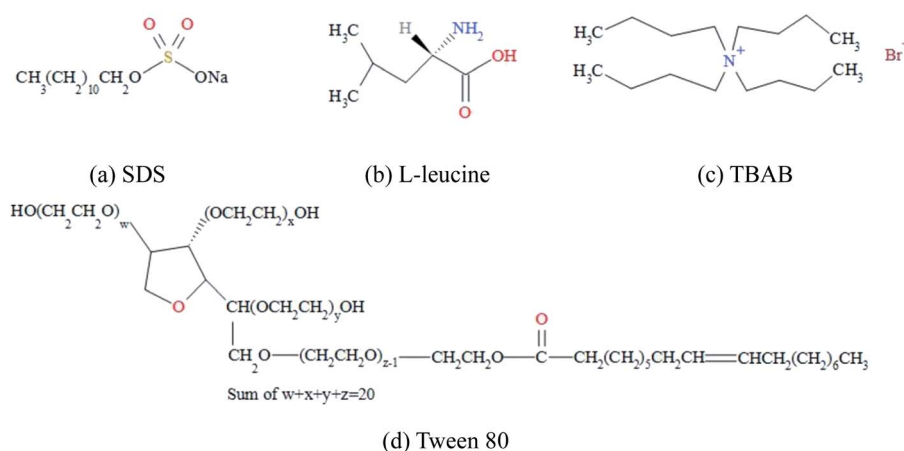
Fig. 1 Chemical structure of four hydrate promoters.
