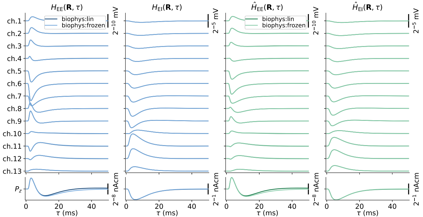
Fig 11. Spike-LFP impulse response function averages and predictions. Similar to panels in Fig 5, but with the excitatory cell model being replaced by a biophysically detailed pyramidal cell model [30].
