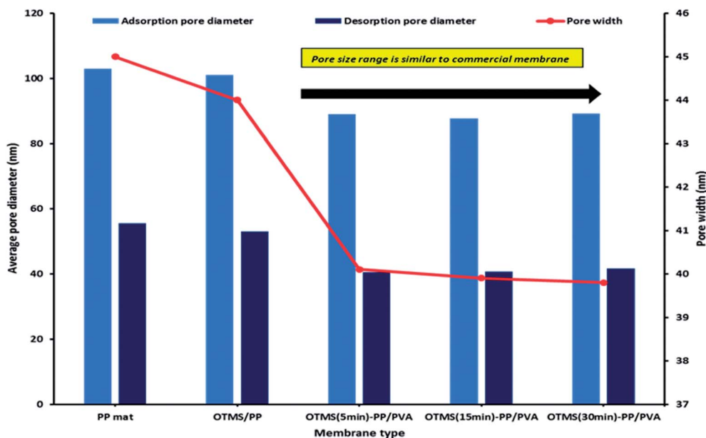
Fig. 8 Barrett–Joyner–Halenda (BJH) analysis of adsorption/desorption average pore diameter and pore width for different modified membranes.
