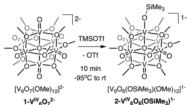
Scheme 1 Synthesis of complex 2-V IV O 6 (OSiMe 3 ) 1– .
