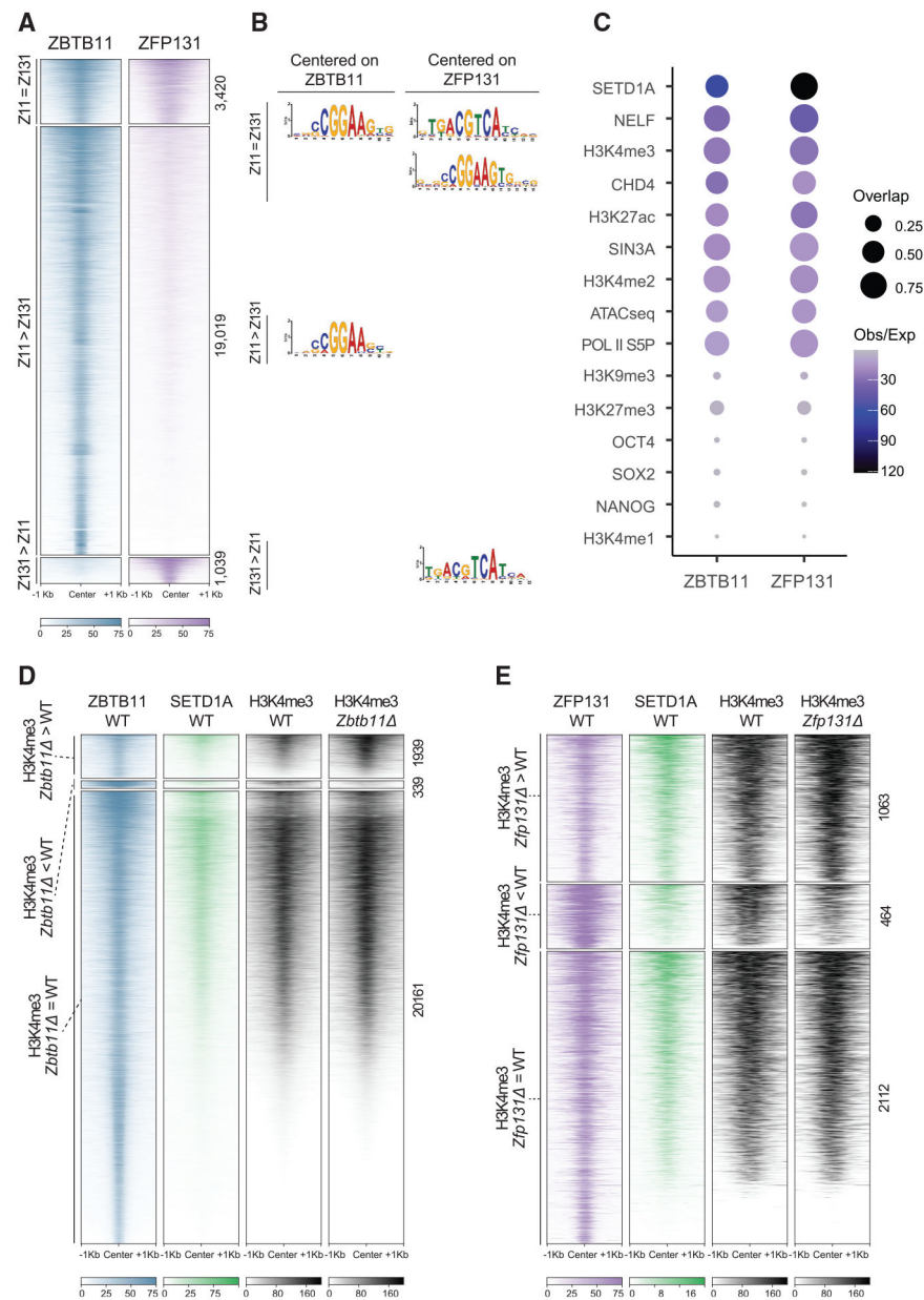
Figure 4. ZBTB11 and ZFP131 bound sites gain an H3K4me3 signal in Zbtb11 and Zfp131 knockout cells
