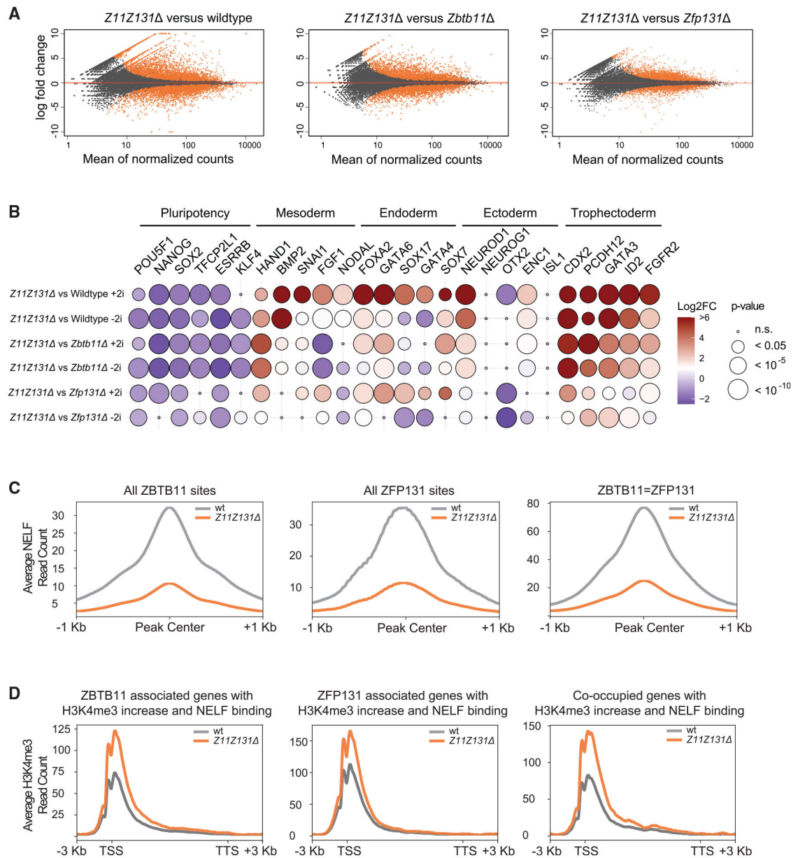
Figure 7. Double-knockout cells further increase pro-differentiation gene expression and H3K4me3 signal
