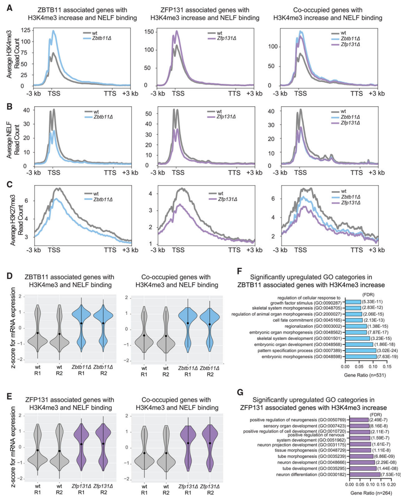
Figure 6. ZBTB11- and ZFP131-associated pro-differentiation genes gained H3K4me3 and lost NELF at TSSs and are transcribed in Zbtb11 and Zfp131 cells
