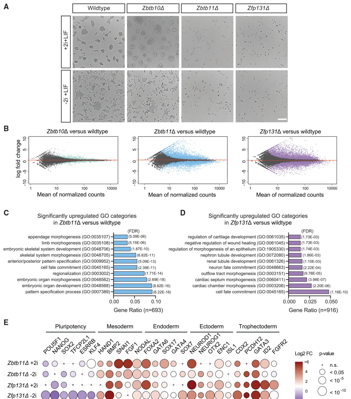
Figure 2. Zbtb11 and Zfp131 knockout cells express genes associated with multiple germ layers (A) Zbtb10 , Zbtb11 , and Zfp131 colony morphology in +2i + LIF and -2i + LIF conditions 3 days after doxycycline removal. Zbtb11 and Zfp131 cells lose typical ESC colony formation ability and adopt morphologies associated with differentiation. Scale bar, 200 \mu m.
