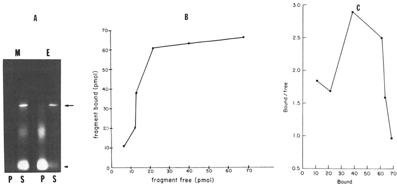
Figure 8. (A) Site specificity in vimentin-membrane interactions. A ^{125}\text{I} -vimentin chymotryptic digest, prepared as described (58 \mu\text{g}/\text{ml} vimentin, 1,700 cpm/ \mu\text{g} ) was co-incubated with plasma membranes (40 \mu\text{g} ) or nuclear envelopes (70 \mu\text{g} ) under standard conditions (assay volume 180 \mu\text{l} ). The resultant pellets and supernates were subjected to electrophoresis in 15% acrylamide gels and autoradiographed. M, plasma membranes. E, nuclear envelopes. P, pellet. S, supernatant. Arrow indicates the 38-kD middle domain of vimentin and the arrowhead, its 6.6-kD domain (photographed in reverse contrast). The relatively heavier labeling of the tail piece is due to the higher accessibility of this peripheral domain to the Bolton-Hunter reagent when concentrated vimentin samples are used. Under these conditions the protein partially assembles during iodination and the coiled-coil regions are apparently protected. With more dilute preparations the labeling is proportional to the number of iodination sites occurring at the 38- and the 6.6-kD domains (more in the former and mainly Lys or His). (B) The binding of the 6.6-kD tailpiece to nuclear envelopes. Assays were executed as in A with increasing quantities of the digest. After electrophoresis the appropriate bands were excised and the radioactivity was determined by \gamma -counting. (C) The same data shown in B after Scatchard analysis.
