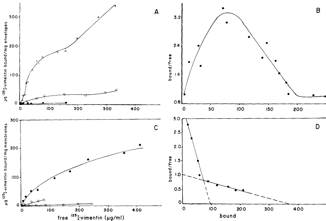
Figure 2. (A) Binding of ^{125}\text{I} -vimentin to phosphate-extracted nuclear membranes ( \Delta ), nuclear membranes before extraction ( \circ ), and trypsinized nuclear membranes ( \bullet ). (B) Scatchard plotting of the data shown in A (the last point of the isotherm is omitted). (C) Binding of ^{125}\text{I} -vimentin to extracted plasma membrane ( \bullet ), trypsinized plasma membranes ( \circ ), or intact erythrocytes ( \diamond ). The milligram equivalent was estimated assuming 10^{-6} µg of membrane protein/cell as calculated from ghost electrophorograms. This value is similar in the order of magnitude with the one calculated for Dogde ghosts of human RBC. (D) Scatchard plotting of the data shown in C. For details see Materials and Methods.
