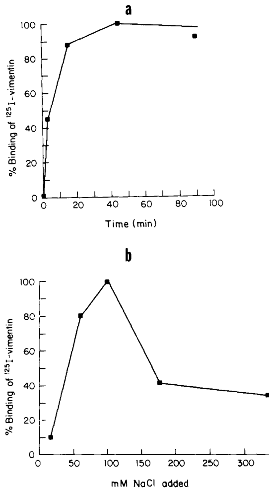
Figure 5. (a) Time course of the binding of 125 I-vimentin to nuclear envelopes. 6 \mu\text{g} of 125 I-vimentin was incubated with nuclear envelopes as specified in Materials and Methods for the time periods indicated on the abscissa. The centrifugation time was not considered for constructing the curve. (b) Salt dependence of the binding of 125 I-vimentin to nuclear envelopes. Experiments were executed as in a in a buffer containing 5 mM NaPO 4 , 0.1 mM PMSF, and 2 mM MgCl 2 pH 7.6 plus the indicated concentrations of NaCl. The maximum binding achieved was considered 100% binding.
