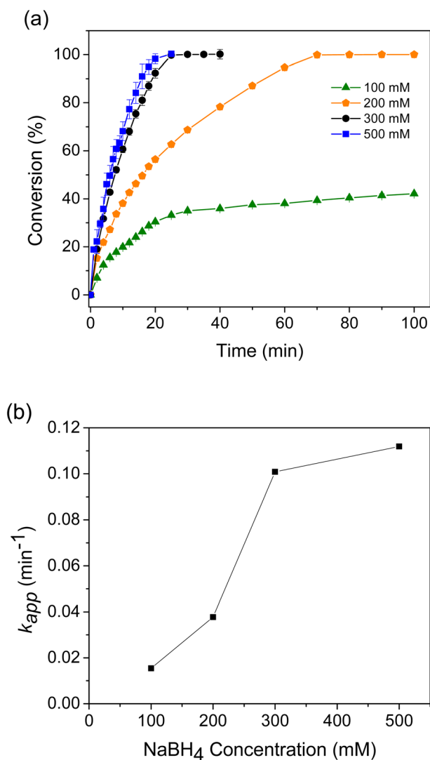
Fig. 7 (a) Effect of NaBH 4 concentration and (b) rate constants for 4-nitrophenol reduction. Condition: [cat.] = 3 g L -1 ; [4-NP] = 15 mM.
