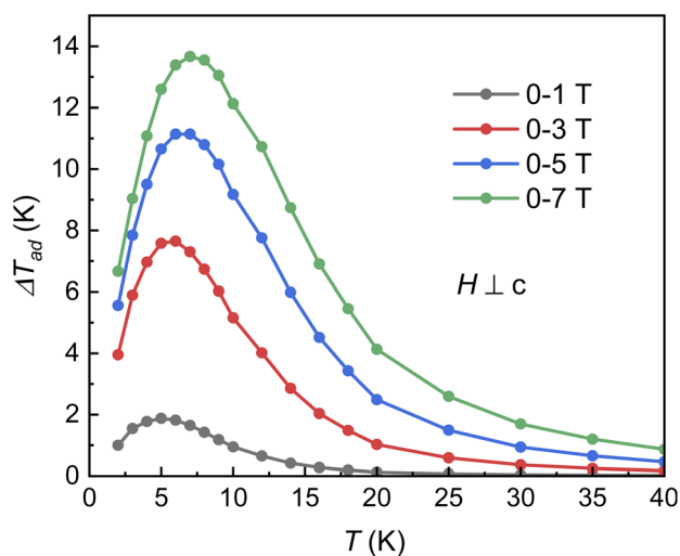
Fig. 7 Temperature dependence of adiabatic temperature change \Delta T_{\text{ad}} .
