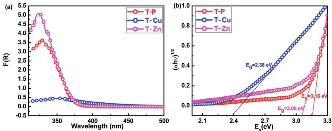
Fig. 6 (a) UV-visible spectra of T-P, T-Cu and T-Zn samples and (b) corresponding Tauc's plot.
