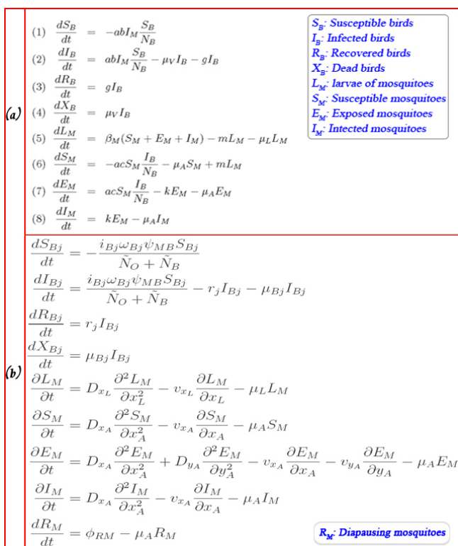
Figure 12 (a) Differential equations of Wonham's mathematical model [16], and (b) the new equations of the proposed model [18].
