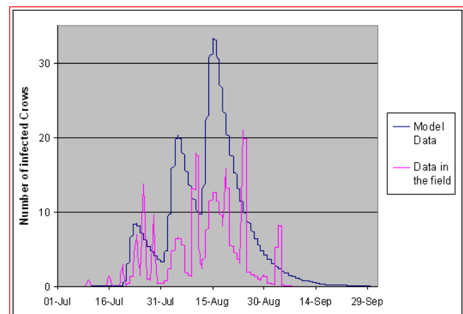
Figure 9 Model calibration using the average collected dead birds during the considered period of the simulation (1 July – 1 October) for Laval Municipality (2003 to 2006).
