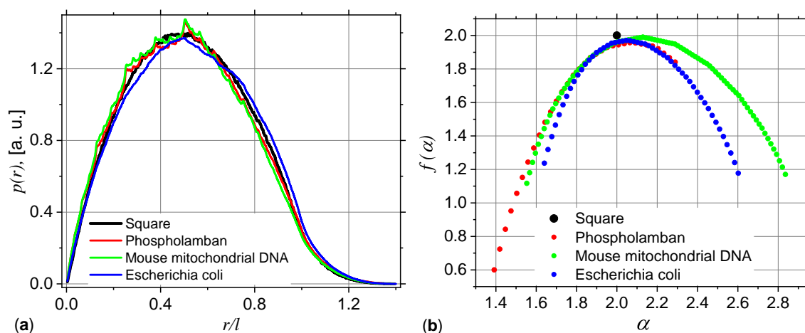
Figure 12. Pddf (a) and f(\alpha) spectra (b) for Phospholamban , Mouse mitochondrial DNA and Escherichia coli . The data for a uniform square are included for comparison.
