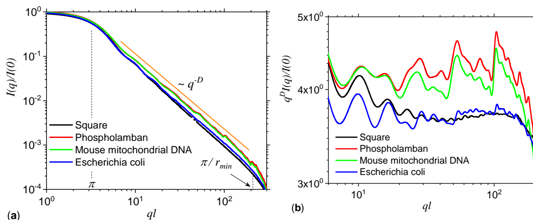
Figure 11. Scattering intensities I(q) (a) and q^D I(q) (b) of Phospholamban (red), Mouse mitochondrion DNA (green), and Escherichia coli (blue). For comparison, the scattering intensity of a uniform distribution of points within a square is shown. l is the overall size of the “ACGT” square, r_{min} is the minimum scale on which the samples have a fractal behavior, and D is the fractal dimension (see text for details).
