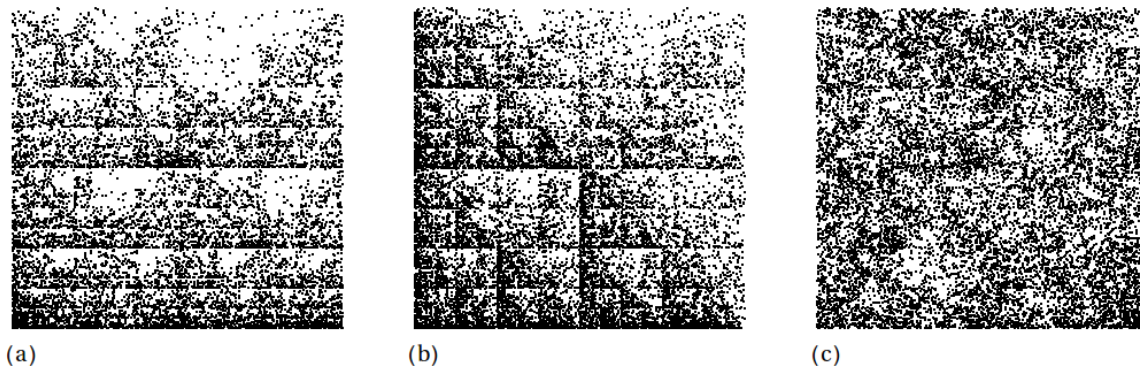
Figure 10. CGR in the “ACGT” square, with A = (0,0) , T = (1/2,0) , G = (1/2,1/2) , C = (0,1/2) for Phospholamban , GenBank ID: 5350 (a), Mouse mitochondrion , GenBank ID: 342520 (b), and Escherichia coli (c), NCBI Accession Version NZ_BJSS01000161.
