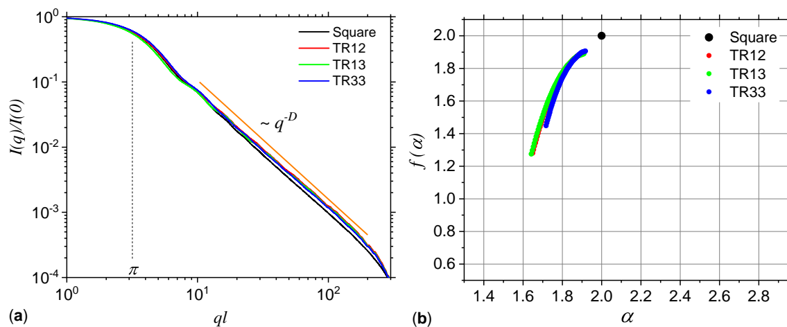
Figure 9. Scattering intensities (a) and f(\alpha) spectra (b) for models TR12, TR13 and TR33. l is the overall size of the “ACGT” square. The data for a uniform square are included for comparison.
