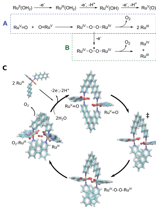
Fig. 5 Putative reaction mechanism of catalyst 3. Oxidation of \text{Ru}^{\text{II}}-\text{H}_2\text{O} yields the \text{Ru}^{\text{V}}=\text{O} species from which the catalysis starts. Catalyst 3 forms a dimeric core complex, and via radical coupling and peroxy \text{Ru}^{\text{IV}}-\text{O}-\text{O}-\text{Ru}^{\text{IV}} intermediate yields \text{O}_2 (pathway A). Under highly oxidizing conditions, the \text{Ru}^{\text{IV}}-\text{O}-\text{O}-\text{Ru}^{\text{IV}} intermediate could be further oxidized to yield \text{O}_2 and a mixed valence \text{Ru}^{\text{IV}}/\text{Ru}^{\text{III}} product state (pathway B). (C) Structure of computed intermediates within putative reaction cycle of catalyst 3.
