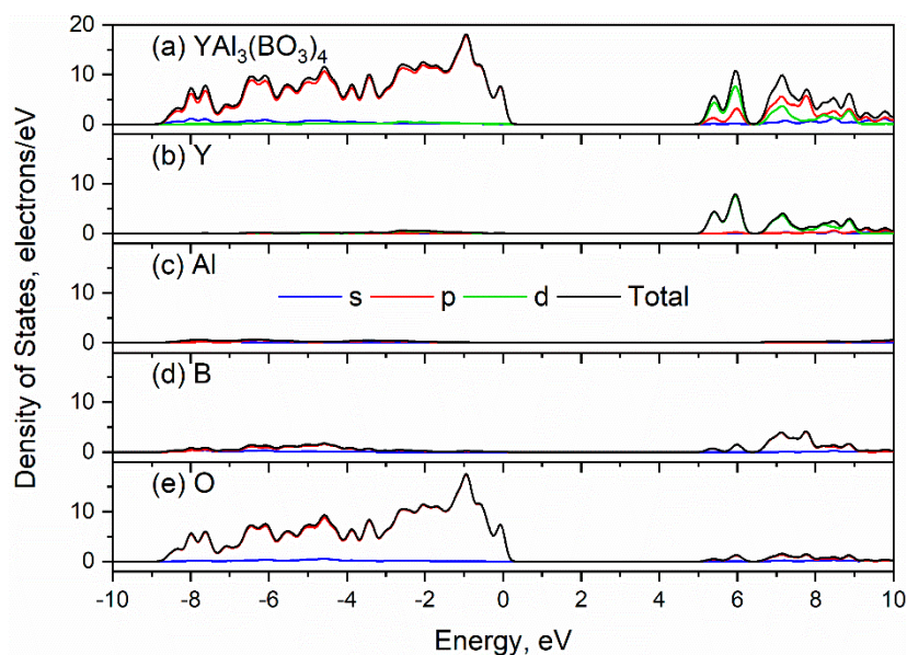
Figure 4. Total (a) and partial density of states (b), (c), (d), (e) of YAl_3(BO_3)_4 .
