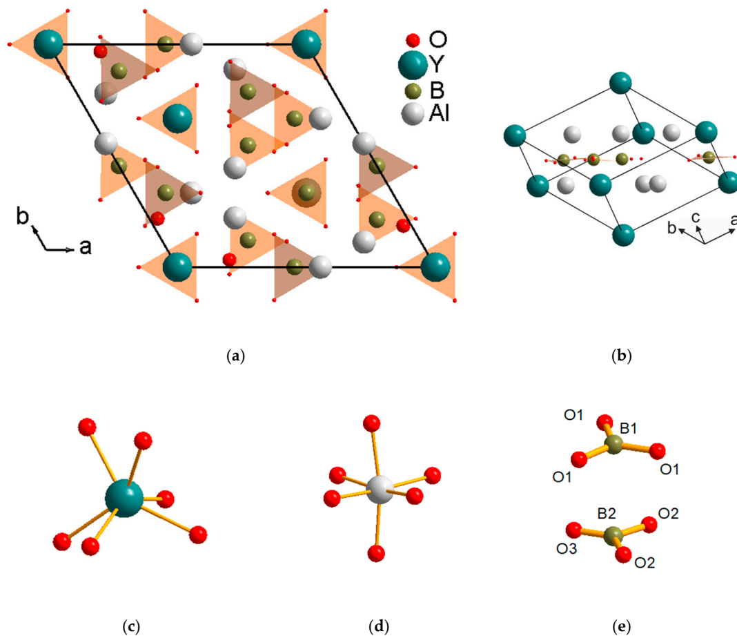
Figure 1. Projection of the YAl_3(BO_3)_4 unit cell on the basal plane (a) and its primitive cell (b). Basic structural units: (c) YO_6 , (d) AlO_6 and (e) BO_3 .
