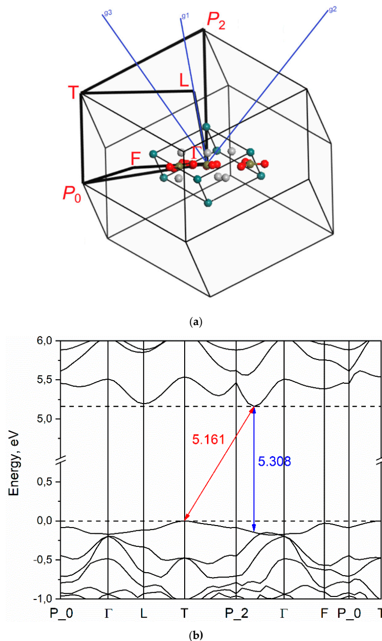
Figure 3. Brillouin zone of the \text{YAl}_3(\text{BO}_3)_4 rhombohedral lattice (a) and electronic band structure (b).
