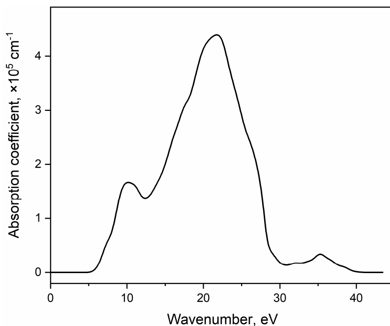
Figure 5. The calculated YAl_3(BO_3)_4 absorption coefficient versus photon energy.
