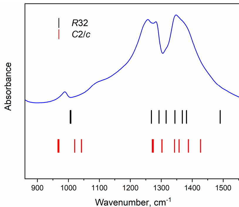
Figure 8. The IR absorption spectra of YAl_3(BO_3)_4 in the range of stretching vibration of BO 3 triangles in comparison with calculated wavenumbers (vertical lines) of IR-active vibrations in trigonal (R32) and hypothetical monoclinic (C2/c) structures.
