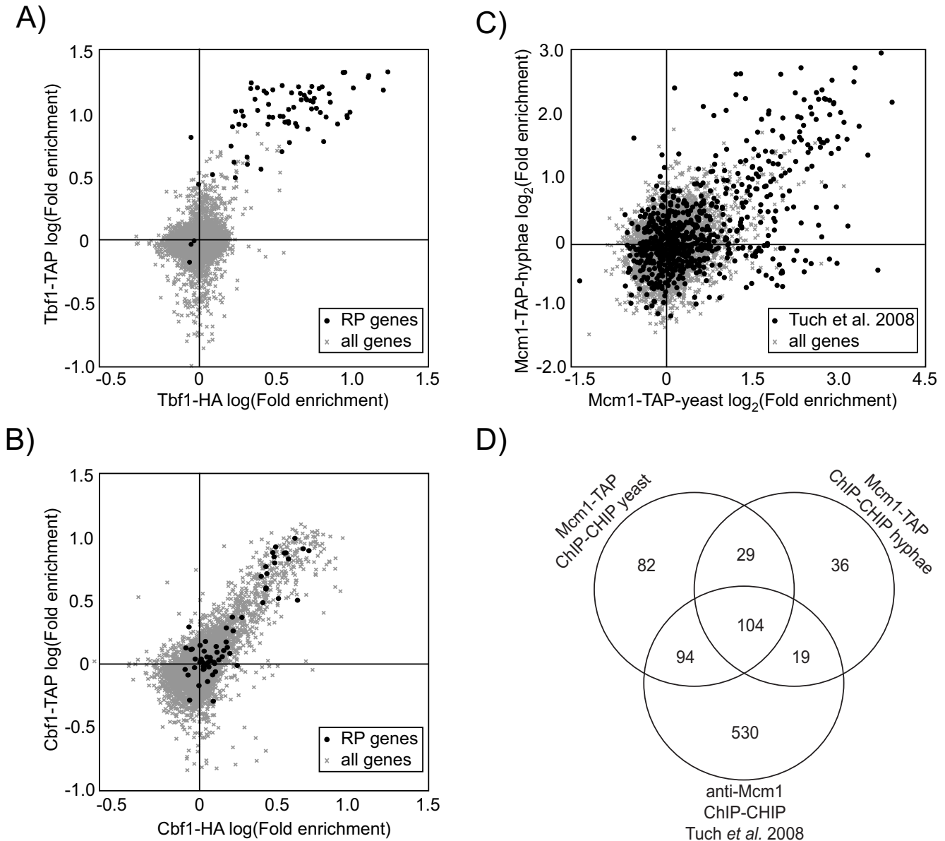
Figure 3 Validation of the Cbf1, Tbf1 and Mcm1 TAP-tagged TFs by ChIP-CHIP analysis. Tbf1-HA and Cbf1-HA ChIP-CHIP [20] overlaps Tbf1-TAP (A) and Cbf1-TAP (B) ChIP-CHIP performed with our in vivo tagged constructs. C) Comparison of Mcm1-TAP ChIP-CHIP conducted before and after the yeast to hyphal transition with the Mcm1 targets derived from Tuch et al. (2008) experiments highlighted. D) Comparison of the target genes of Mcm1-TAP in yeast and hyphal states and their overlap with Tuch et al. (2008) gene list.
