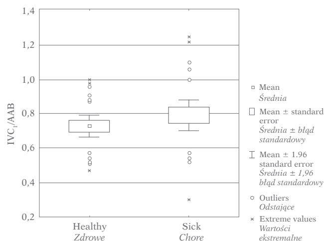
Fig. 5. Box plot: Whiskers for the groups of healthy and sick neonates for IVC_1/AAB values
