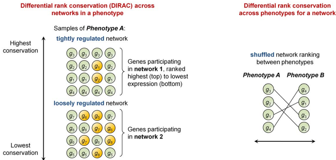
Figure 2. Prototypical scenarios observed for networks in DIRAC. doi:10.1371/journal.pcbi.1000792.g002
