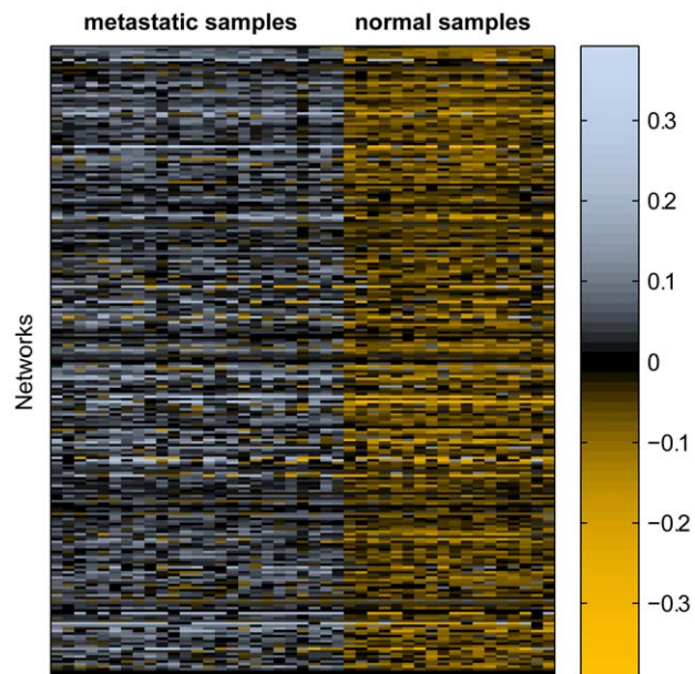
Figure 6. Differential rank conservation across all networks for a set of two prostate phenotypes. Positive rank difference scores predict a metastatic sample and negative difference scores predict a sample as normal.
