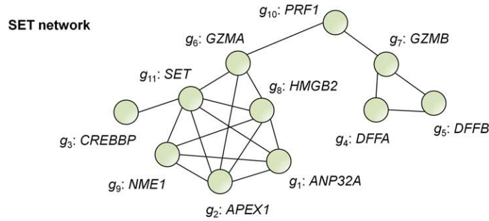
Rank conservation of SET pathway in normal prostate
