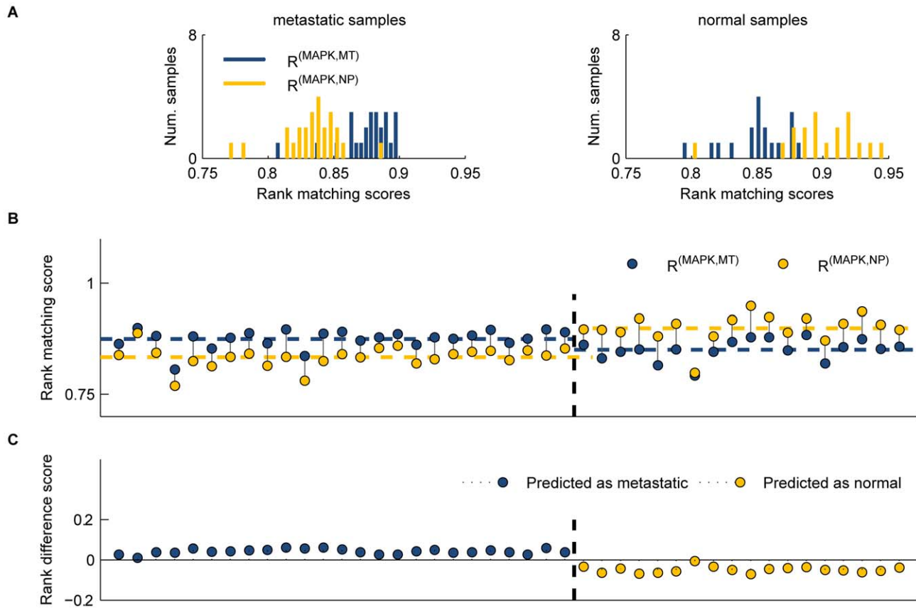
Figure 7. Differential rank conservation of the MAPK network in metastatic prostate cancer and normal prostate. (A) Histograms of rank matching scores. MT template matching scores ( R^{(MAPK,MT)} ) are higher on average in MT samples than NP matching scores ( R^{(MAPK,NP)} ). In NP samples, R^{(MAPK,NP)} scores are higher on average than R^{(MAPK,MT)} scores. (B) Rank matching scores for the MAPK network. Comparing the two rank matching scores in each sample, MT samples are more similar to the MT template than to the NP template in all cases; NP samples are ranked more similarly to the NP template more than the MT template in all cases. (C) Rank difference score values for the MAPK networks. Samples are classified as MT if the rank difference score is greater than zero and as NP if the difference is less than zero. doi:10.1371/journal.pcbi.1000792.g007
