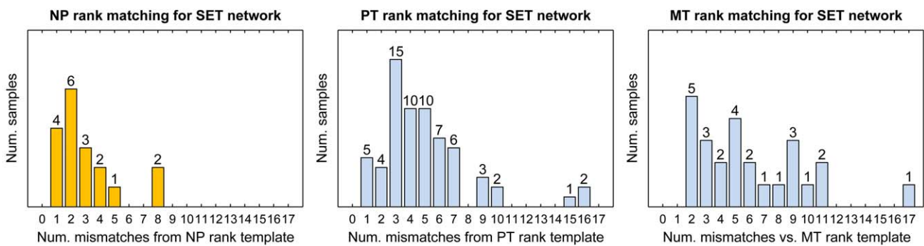
Figure 3. Example of a tightly regulated network in normal prostate. A simplified diagram of the SET network, comprising 11 signaling proteins involved in granzyme mediated apoptosis, is shown in the center. The NP rank template for the network is highlighted yellow, and each unique ranking observed in NP samples is shown to the right with mismatches highlighted red. The histograms at the bottom demonstrate the increased variation in ranking in PT and MT, indicated by greater number of mismatches from the respective rank templates. doi:10.1371/journal.pcbi.1000792.g003
