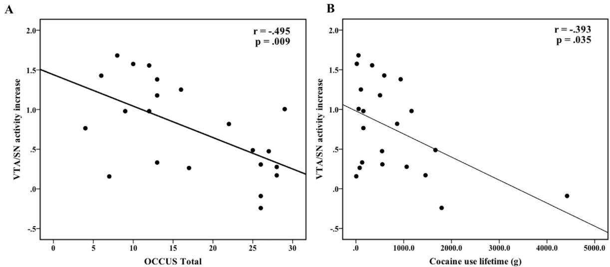
Fig. 3. Spearman correlation of the reward imagery contrast estimate (“Happy Time”–“Rest”) with (A) severity of obsessive-compulsive thought about cocaine (OCCUS Total score) and (B) lifetime cocaine consumption (in g).
